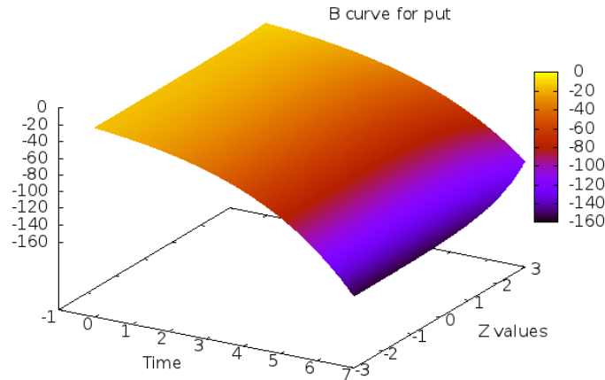
Figure 8.8: The value function b(t, z) for an at-the-money put option.
