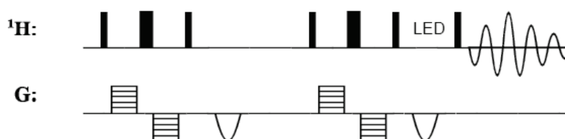
Figure 25. DOSY pulse sequences.
