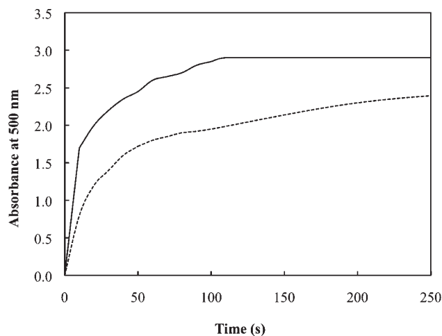
Figure 2. Evolution as a function of time of the ligand exchange reaction COD-CYD for [\text{Rh}(\text{COD})(\text{PPh}_3)_2]\text{NTf}_2 in [\text{C}_1\text{C}_4\text{Im}][\text{NTf}_2] (full line) and [\text{C}_1\text{C}_1\text{C}_4\text{Im}][\text{NTf}_2] (dashed line) monitored at \lambda = 500 nm by UV-vis spectroscopy. UV-visible spectra of [\text{Rh}(\text{COD})(\text{PPh}_3)_2]\text{NTf}_2 and [\text{Rh}(\text{CYD})(\text{PPh}_3)_2]\text{NTf}_2 are provided in the Supporting Information (Figures S-1 and S-2).
