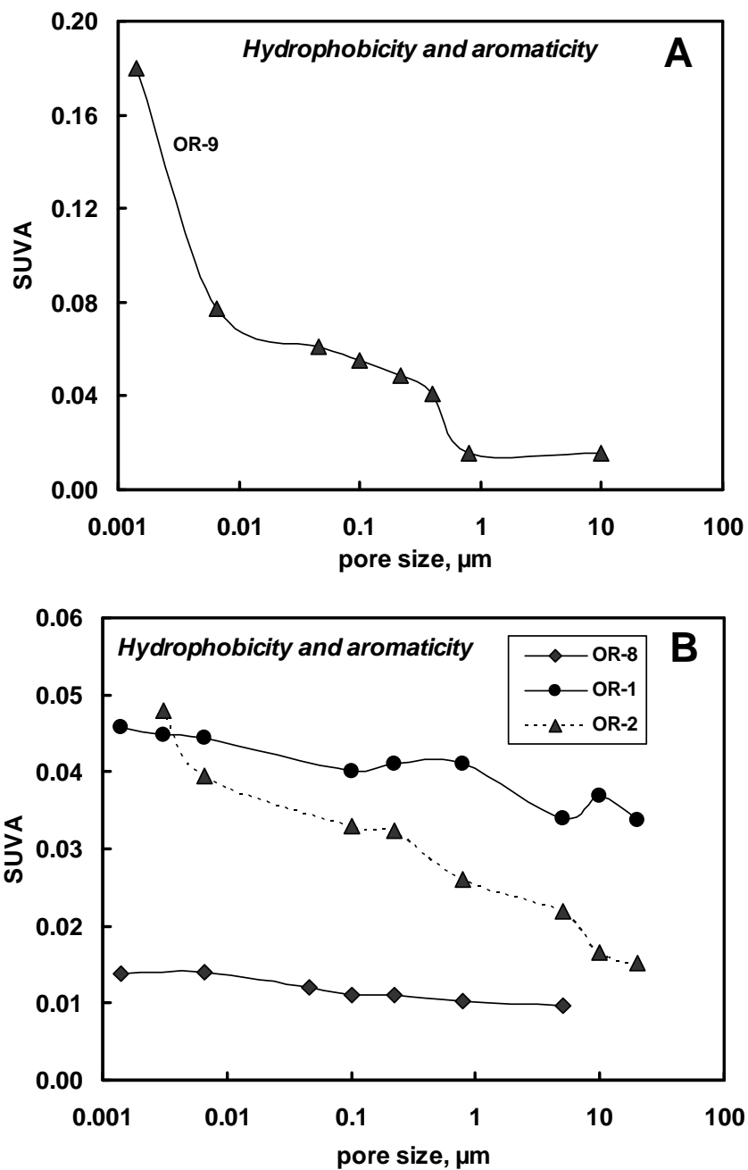
Figure 2.11. SUVA ratios with respect to molecular size fractions for the samples of Vostochniy stream (OR-9 – soil solution, OR-6 – top feeding lake, OR-2 – waterlogged shore of the low feeding lake, OR-1 – mouth reach of the stream, OR-8 – terminal lake).
