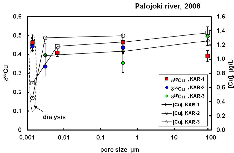
Figure 4.6. \delta^{65}\text{Cu} and Cu concentration as a function of pore size in Palojoiki river waters, KAR-3: a mouth reach, KAR-1: middle course, KAR-2: feeding bog, Karelia. Open symbols – concentrations, closed symbols – isotopic ratios.
