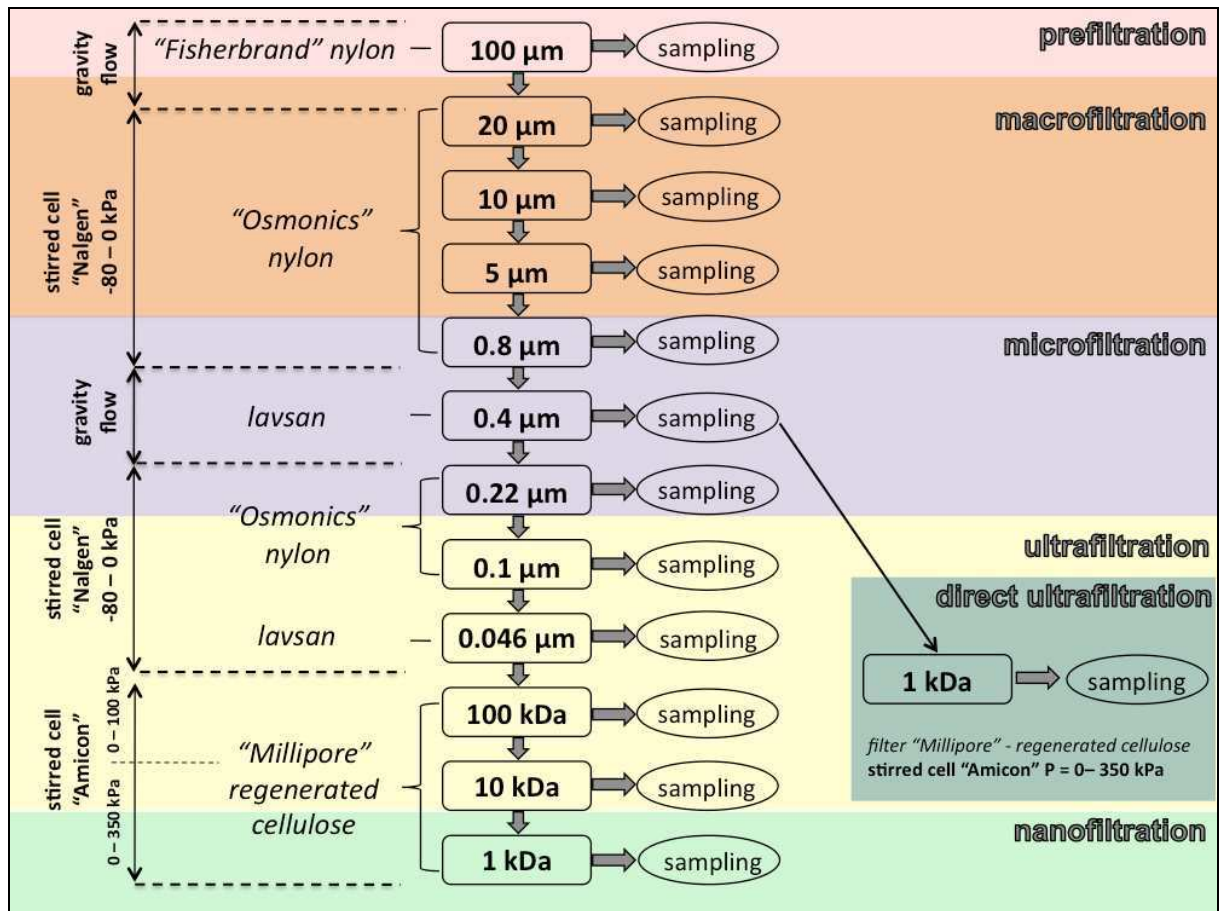
Figure 5.2. The scheme of cascade filtration used in this study. Lavsan is the trade name for polyethylene terephthalate fibers.
