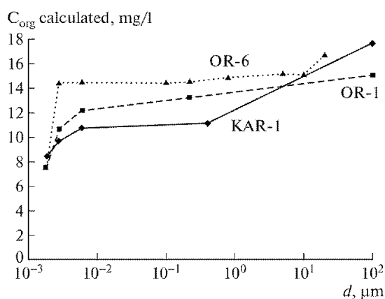
Fig. 6. Distribution of C_{\text{org}} by the filtrates of the samples: KAR-1 is the average flow of the Palojoki River; OR-1 is the mouth of the Vostochniy Stream; OR-6 is the upper lake of the Vostochniy Stream (2009).
