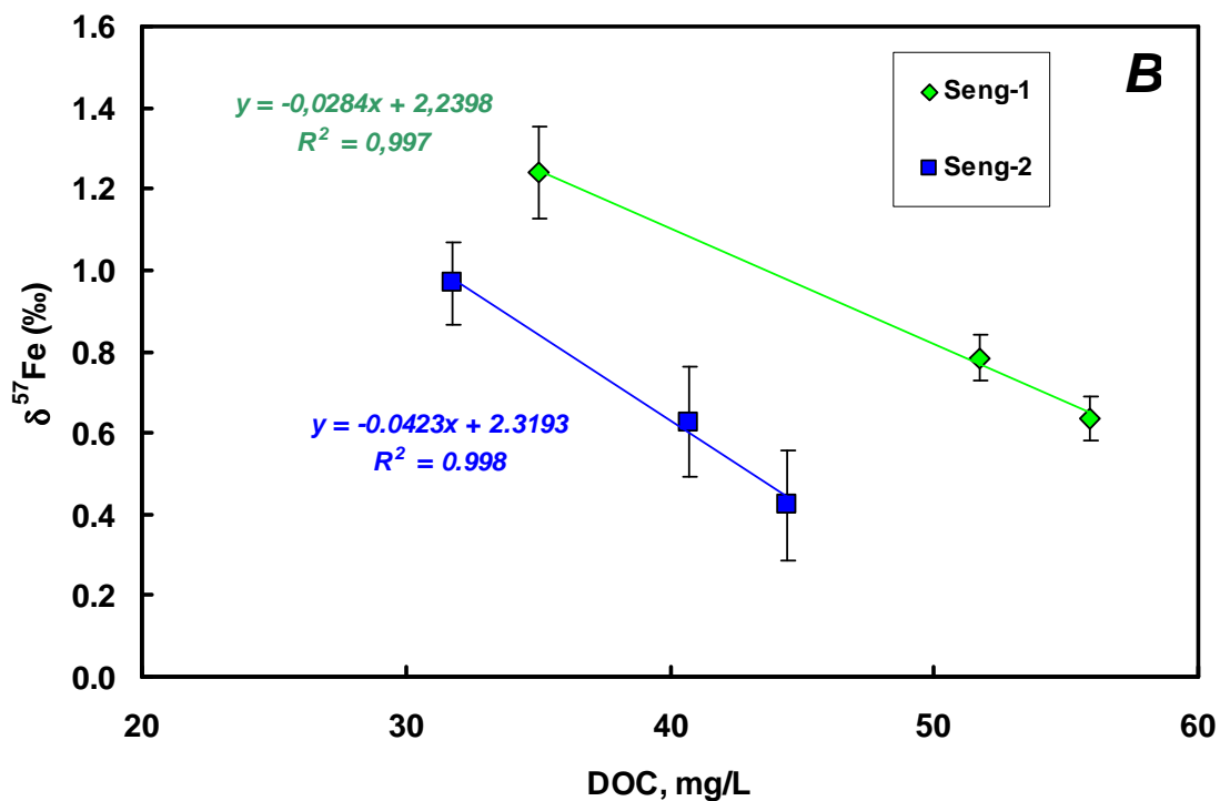
Figure ESM-5.6. \delta^{57}\text{Fe} as a function of DOC concentration in filtrates of organic-poor waters (A) and organic-rich waters (B). OR-1 is mouth reach of Vostochniy stream, OR-6 is feeding lake of Vostochniy stream basin, KAR-1 is middle course of Palojoki river, Seng-1 is mouth reach of Senga river, and Seng-2 is middle course of Senga river.
