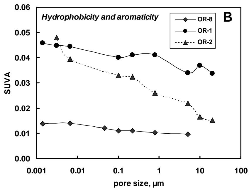
Figure 2.11. SUVA ratios with respect to molecular size fractions for the samples of Vostochniy stream (OR-9 – soil solution, OR-6 – top feeding lake, OR-2 – waterlogged shore of the low feeding lake, OR-1 – mouth reach of the stream, OR-8 – terminal lake).
