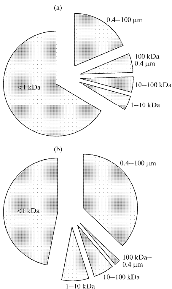
Fig. 7. Distribution of C_{\text{org}} in selected filtrates of the sample of the average flow of the Palojoki River: (a) KAR-1/08, July, 2008; (b) KAR-2/09, August, 2009.
