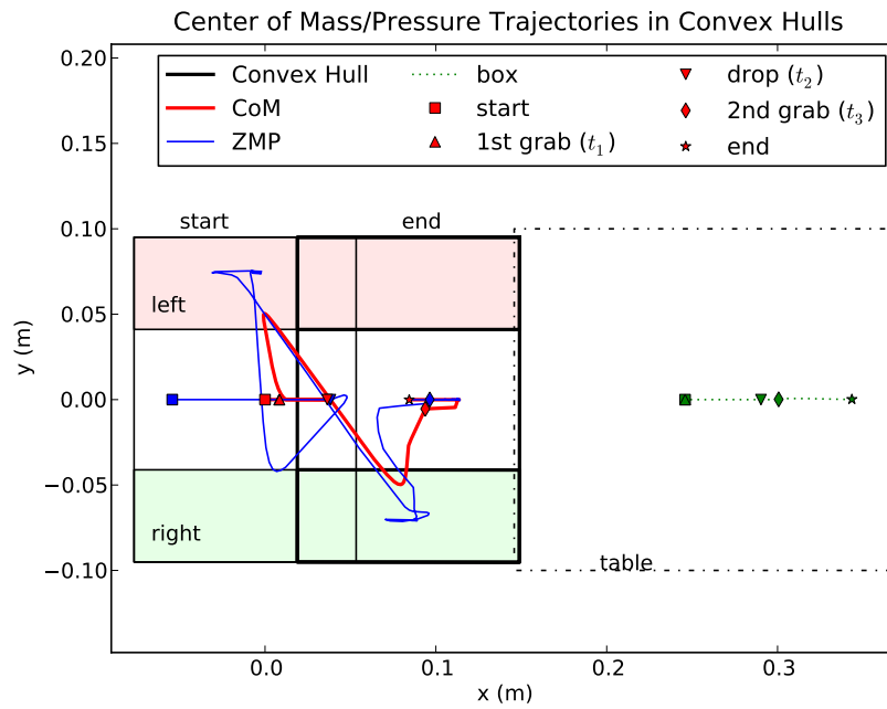
FIGURE 4.12.: Experiment 4, second case – Trajectories of the ground projections of the CoM position (plain bold red), ZMP position (plain blue) / Box positions (dashed green) / Foot placement (colored zones) and convex hulls (plain black) before and after corrective actions.
