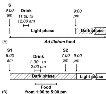
Fig. 2. Schematic representation of the daily schedule of the baseline (A) and detection (B) experiments. In the first experiment, the rats were fed ad libitum and placed under a 23 h-water deprivation schedule (A). The daily experimental session (S) was performed at 9:00 a.m. In the second experiment, the rats were under a 23 h-water and a 20 h food deprivation schedule (B). Food was available 4 h per day from 1:00 to 5:00 p.m. Two daily experimental sessions S1 and S2 were performed at 9:00 a.m. and 7:00 p.m. during which the same ISO concentration was presented.
