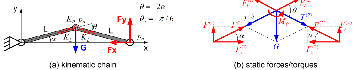
Figure 5.12 Kinematic chain with compliant links and actuator and its static forces/torques
