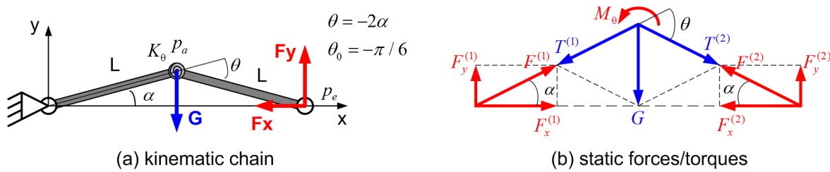
Figure 5.9 Kinematic chain with compliant actuator between two links and its static forces/torques
