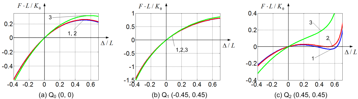
Figure 4.8 Force-deflection relations F = f(\Delta / L) in critical points: (1) K_g = 0 , (2) K_g = 0.05 K_\theta L^2 , (3) K_g = 0.1 K_\theta L^2
