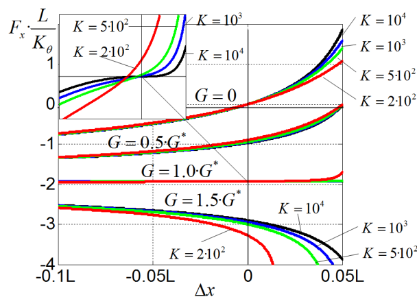
Figure 5.13 Force-deflections relations for different values of auxiliary loading G : chain with torsional and translational springs ( G^* = 4K_0 / L \cdot \sin \alpha_0 , K_L = K \cdot K_0 / L^2 )
