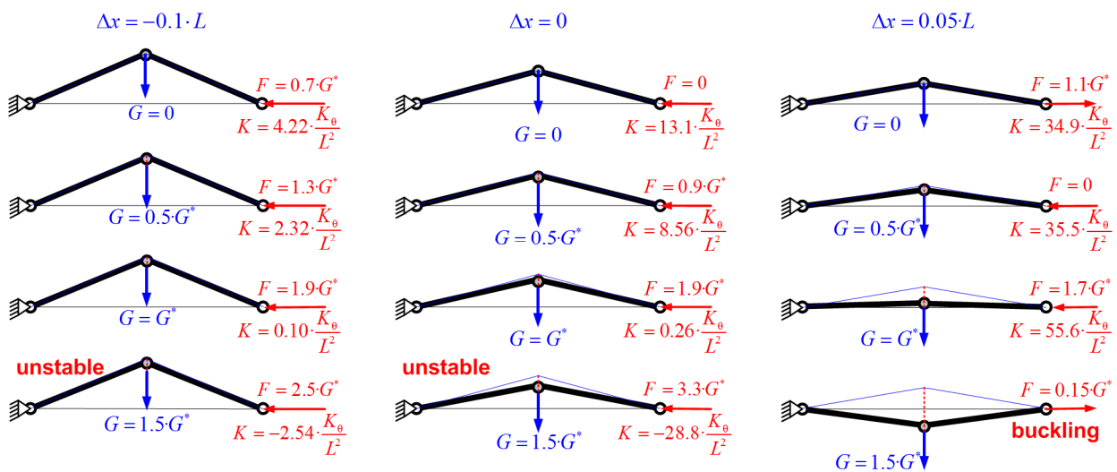
Figure 5.14 Configuration of kinematic chain with auxiliary loading: case of torsional and translational springs ( G^* = 4K_0 / L \cdot \sin \alpha_0 , K_L = 2 \cdot 10^2 \cdot K_0 / L^2 )
