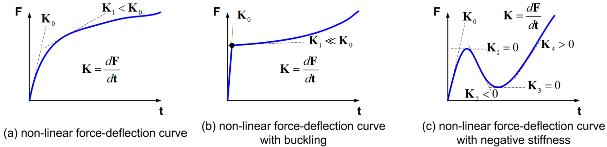
Figure 5.1 Examples of non-linear force-deflection curves
