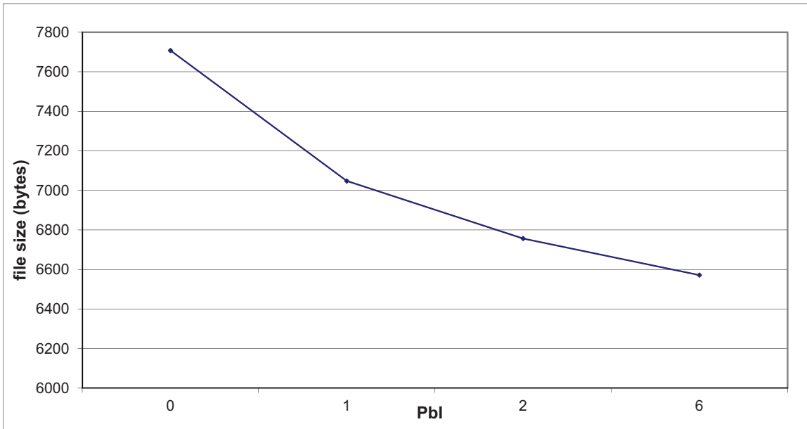
Figure 68. Dependency of the file size with respect to PbI (expressed in segments of 16 frames) for DCT-encoding.
