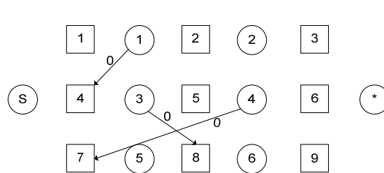
Figure 4-30. Arcs C(7)
