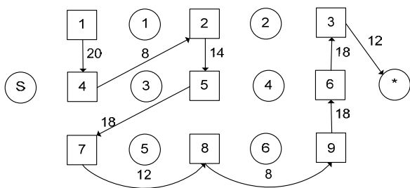
Figure 4-29. Arcs C(3)
