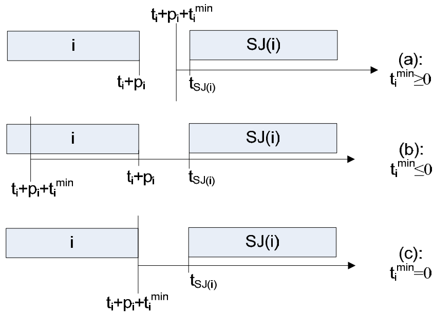
Figure 3-2. Time lag minimum - time lag positif
