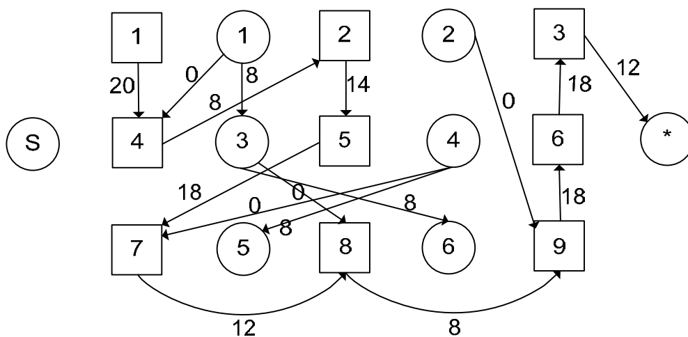
Figure 4-31. Arcs C(4)
