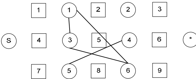
Figure 4-26. Arcs C(2)
