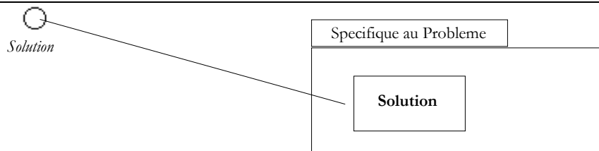
Figure 5-9. Solutions
