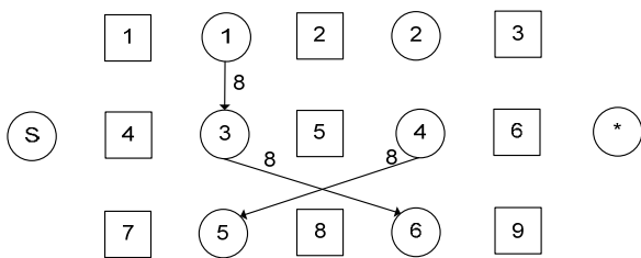
Figure 4-31. Arcs C(4)
