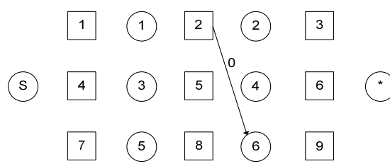
Figure 4-32. Arcs C(8)
