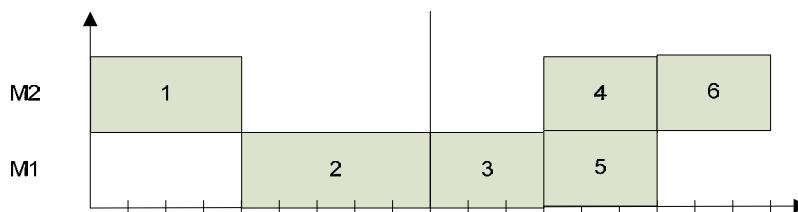
Figure 3-14. Ordonnancement canonique
