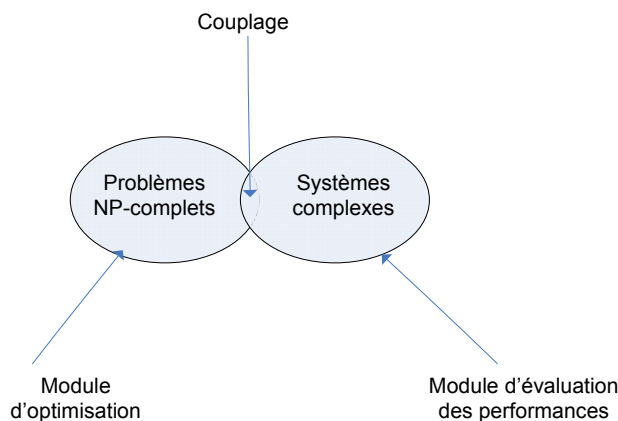
Figure 1-16. Double complexité
