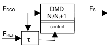
Fig 3: Behavioral model of the D flip-flop by a DMD controlled by the phase error
