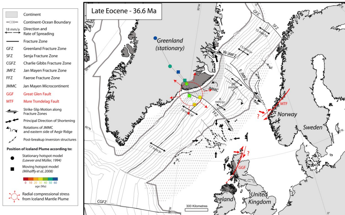
Figure 5.1. Positions, relative to a stationary Greenland plate, of Europe, Jan Mayen Microcontinent and Iceland Mantle Plume, at 36.6 Ma (Late Eocene). Left-lateral slip along FFZ and JMFZ, due to differential spreading along NE Atlantic and possibly to radial compressional stress from Iceland Mantle Plume, could reactivate right-laterally continental lithospheric faults, such as Great Glen Fault, in Scotland and Møre Trøndelag Fault, in Norway.
