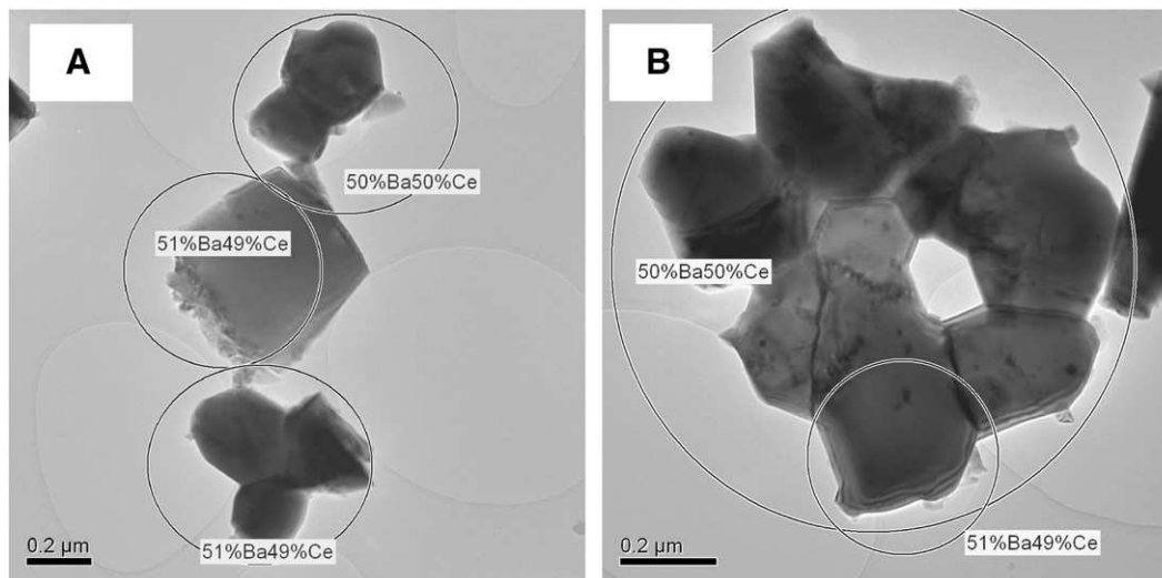
Fig. 4. Transmission electron microscopy analyses of \text{BaCeO}_{3-\delta} ceramic powder: EDX local chemical analyses on individual crystallites are shown in inserts. Ratio Ba/Ce close to 1. Size distribution: D_{\text{TEM}} = 300 \pm 100 nm.
