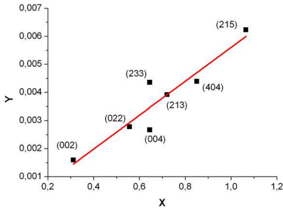
Fig. 6. Williamson–Hall plot for BaCeO 3 sample delivering crystal sizes and distortions: D = 233 ± 100 nm, \epsilon_{(hkl)} = 0.003 \pm 0.0006 .
