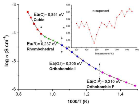
Fig. 8. Logarithm of conductivity ( \log \sigma ) as a function of 10^3/T , with T in Kelvin. Four domains can be observed. Insert figure shows to the evolution of the n exponent of CPE term.
