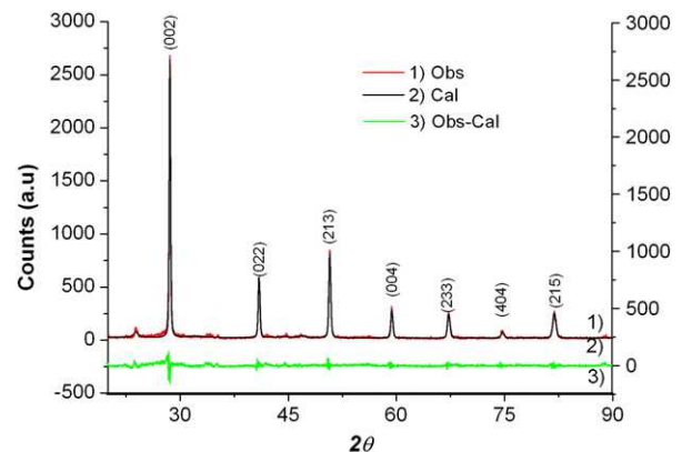
Fig. 5. Rietveld analysis of X-ray diffraction patterns for \text{BaCeO}_{3-\delta} ceramic powder.
