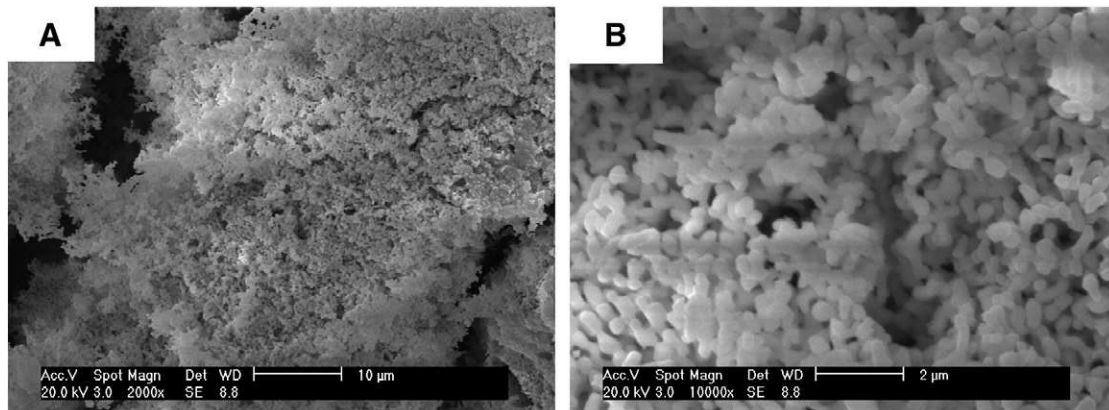
Fig. 3. Scanning electron microscopy images of BaCeO 3-δ ceramic powder using the modified EDTA–citrate method. Amplified (A) 2000x and (B) 10000x.
