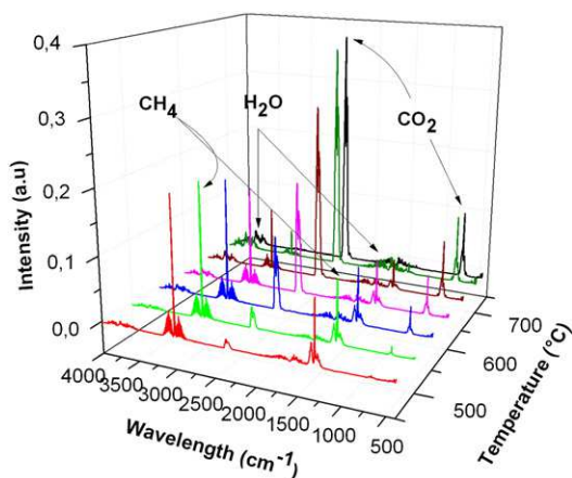
Fig. 9. FTIR spectra evolution of the \text{CH}_4 and \text{CO}_2 absorption bands, as a function of temperature (selection of spectra).
