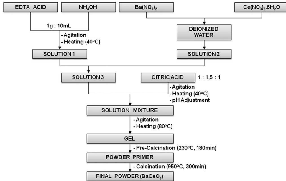
Fig. 2. Flowchart illustrating the preparation process of BaCeO 3-δ powder using the modified EDTA–citrate complexing method.
