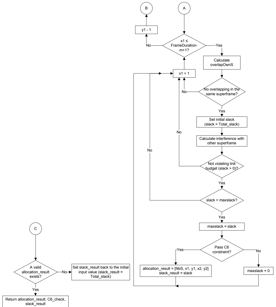
Figure C.4: Minimum interference part 2.
