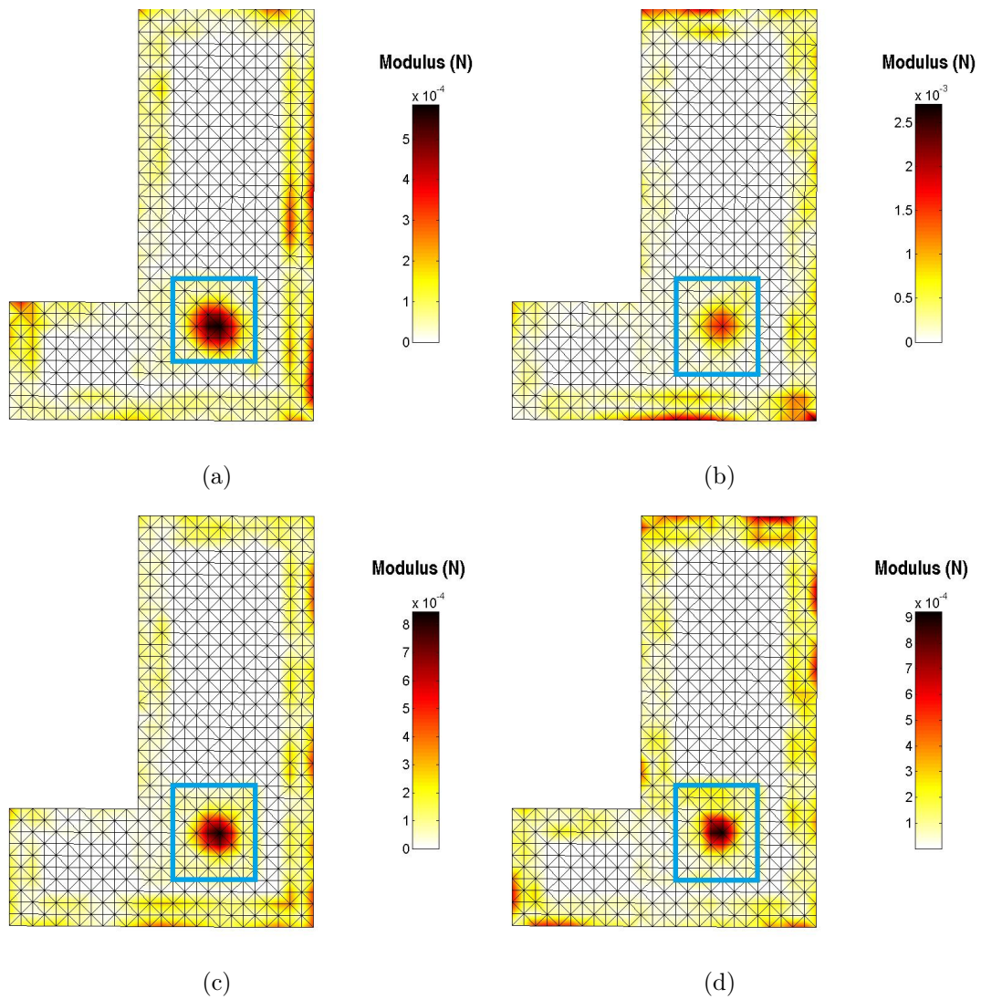
FIGURE 3.18 – Colormap of the amplitudes of the forces \mathcal{F}^{\text{rectikh}} identified on the plate from experimental measurements. 16 fixed interface modes kept to estimate the reduced subdomain. (a) f = 560\text{Hz} ; (b) f = 750\text{Hz} ; (c) f = 1040\text{Hz} ; (d) f = 1475\text{Hz} .
