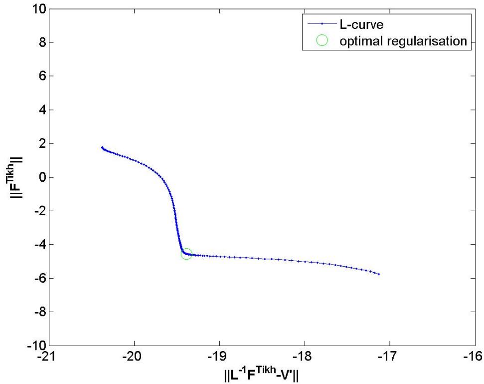
FIGURE 2.17 – L-curve obtained at f = 400 Hz. \|\mathbf{F}^{\text{tikh}}\| is the 2-norm of the solution vector while \|\mathbf{L}^{\text{pinv}}\mathbf{F}^{\text{tikh}} - \mathbf{V}^m\| is the 2-norm of the residue. Input data are measured and injected into the Finite Element model of the whole structure by using the observation matrix from Equation (2.5). The Tikhonov regularisation is used.
