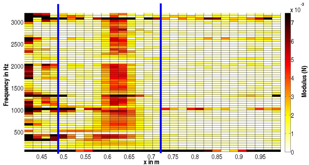
FIGURE 4.8 – Colormap of the magnitude of the computed forces applied by the shaker.
