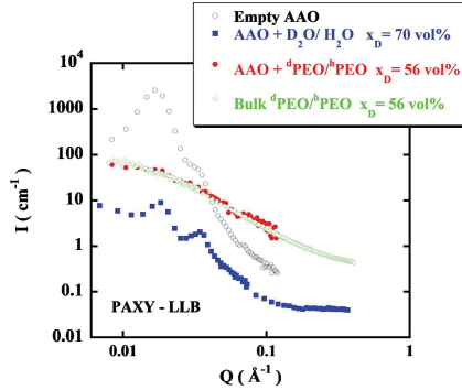
FIG. 2. (Color online) SANS spectrum of an empty AAO membrane. The extremely intense peak at 1.7 \cdot 10^{-2} \text{ \AA}^{-1} is characteristic of the inter pore distance, here D_{int} = 370 \pm 40 \text{ \AA} . The pore diameter is D_p = 180 \pm 20 \text{ \AA} . The neat AAO membrane intense signal can be nearly perfectly matched [11] upon membrane impregnation by an isotopic mixture of water ( x_D = 70 \text{ vol \%} ) or PEO ( x_D = 56 \text{ vol \%} ). In the later case, the remaining contribution is the form factor of a single polymer chain. No large scale structural differences between the bulk and confined chain conformation are detected.
