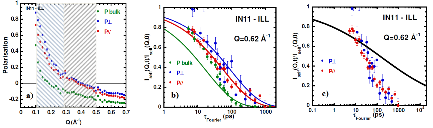
Figure 2.10. NSE results. The sample is ^h PEO ( M_w = 35000 \text{ g.mol}^{-1} ) confined within the macroscopically oriented structure of an AAO (24 nm in diameter), at 373 K. AAO membranes being macroscopically oriented, orientation of the sample in the neutron beam makes it possible to access the dynamics parallel and perpendicular to the pores. a) Polarization of the neutron beam for bulk PEO, and for the two orientations of the AAO confined sample. b) Neutron Spin Echo measurements (IN11-ILL) of I_{Self}(Q, t) Eq. 2.3, the self intermediate scattering function, at Q = 0.62 \text{ \AA}^{-1} . No differences between the polymer dynamics perpendicular (blue symbols) and parallel (red symbols) to the axis of the cylindrical AAO pores are detected. The analytic calculation Eq. 2.14 of I_{Self}(Q, t) in the case of the corset effect, namely a diameter of the reptation tube as low as d_{Rep} = 0.6 \text{ nm} is plotted as a full black line. The significant discrepancy between this theoretical curve and the experimental data lead to the conclusion that we do not observe the corset effect, instead the confined PEO dynamics is similar to the behavior in bulk i.e. the Rouse behavior holds. From [57].
