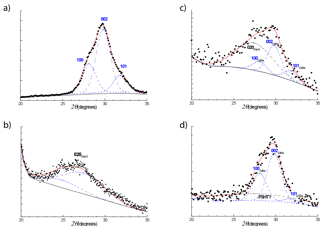
FIGURE II.25 – Zooms of the grazing incidence X-ray diffractograms We focus on the 20^\circ - 35^\circ 2\theta range of the X-ray profiles of a) CdSe nanopods only (powder diffractogram); b) pristine P3HT2; c) hybrid based on P3HT2 and 16 vol% of pyridine-treated nanopods; d) hybrid based on P3HT2 and 16 vol% of nanopods capped with their synthesis ligands. Films on b) and d) were drop-cast from ODCB, the film on c) from ODCB:pyridine 19:1.
