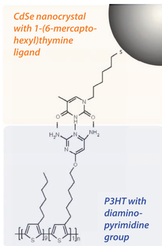
FIGURE II.19 – Triple hydrogen bonding between specifically functionalized nanocrystals and functionalized P3HT This system was developed and optimized by Julia De Girolamo [96] and used for dip-coating of hybrid thin films.
