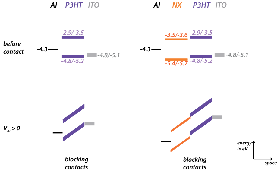
FIGURE IV.4 – Energy diagram of devices for P3HT-only devices and hybrid devices, in the uniform electric field representation. Energy levels were obtained from electrochemistry or from the literature. The width of the lines is an indicator of the range of values found (depending on the size of nanocrystals or on the source).
