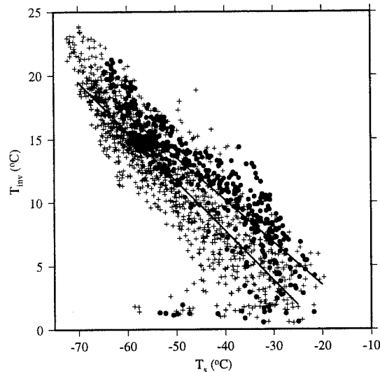
Figure 6.7: T_{inv} as a function of T_s (in °C) for the grounded parts of the Antarctic ice sheet. Full circles: PD; crosses: LGM. Linear regression lines are drawn for both simulations. The linear correlation coefficients r^2 are 0.72 for AA0 and 0.79 for AA21.
