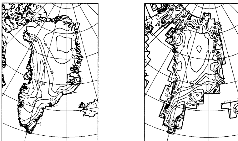
Figure 6.21: Left: Observed present-day annual mean accumulation (after Friedmann et al. [1995]); Right: simulated surface mass balance. Units: cm w.e. yr -1 . Contour lines are -20, -10, 0, 10, 20, 30, 40, 50, 75, 100, 125, 150, and 200 cm w.e. yr -1 .
