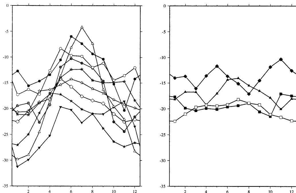
Figure 8.5: The monthly mean surface air temperature change T_{21kyr} - T_{0kyr} in °C for the Greenland grid points above 2000 m. (a) For the models which simulate a clear seasonality; (b) for the models which do not simulate a clear seasonality. Full circles: LMDz GL21PC; Gray circles: LMDz GL21RC; Empty circles: LMDz GL21PW; Full triangles: LMCELMD5; Empty triangles: LMCELMD4; Full diamonds: GENESIS2 with calculated SSTs; Empty diamonds: GENESIS2 with prescribed SSTs; Gray diamonds: GENESIS1; Gray stars: MRI2; Empty stars: UKMO with calculated SSTs; Full stars: GFDL; Inverted full triangles: ECHAM3; Full squares: UGAMP with calculated SSTs; Empty squares: UGAMP with prescribed SSTs; Inverted empty triangles: CCSR1; Hexagons: CCM1.
