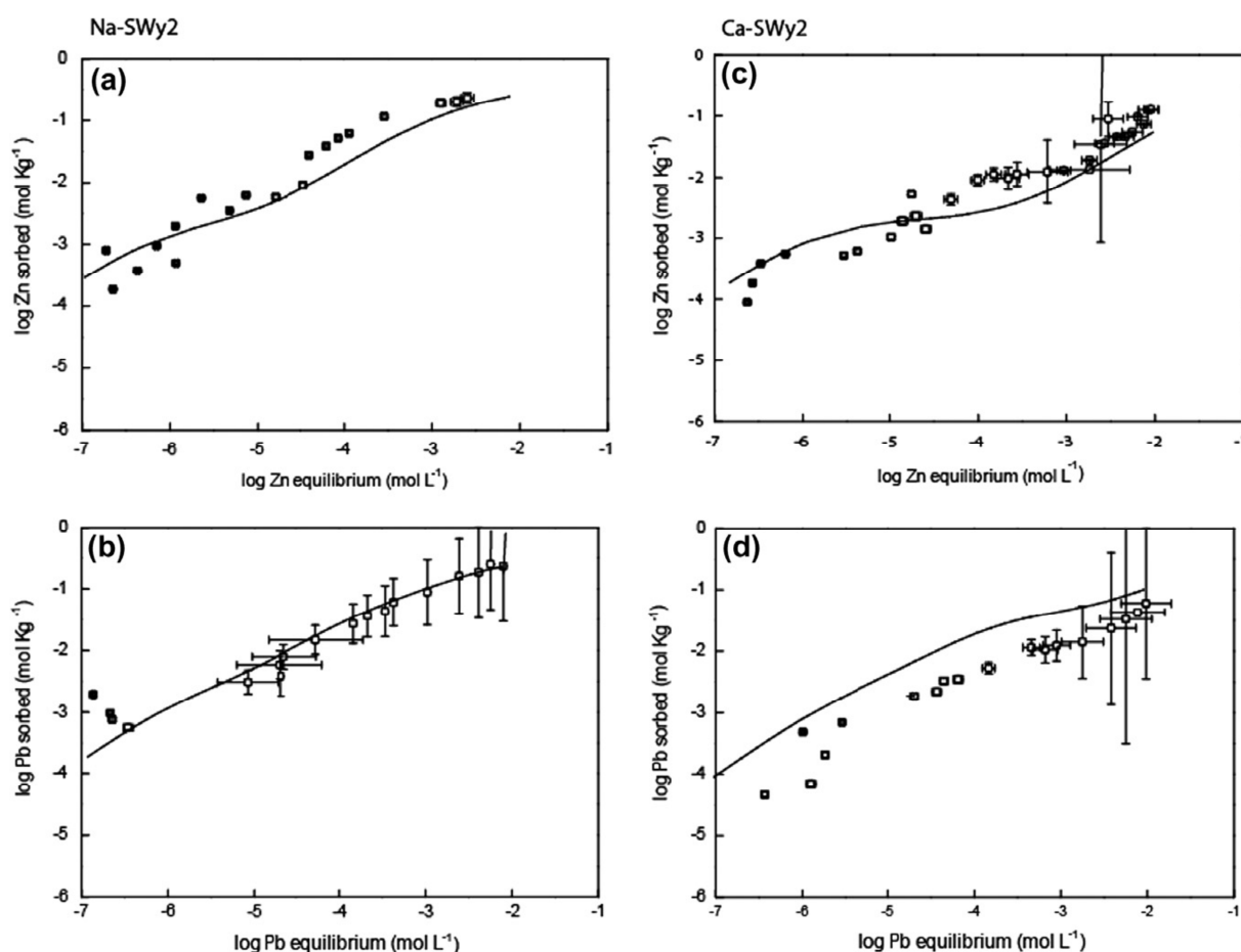
Fig. 2. Metal adsorption isotherms onto montmorillonite at pH = 5, fixed ionic strength ( I = 0.04 \text{ M} ), and low buffer concentration ( 0.001 \text{ M CH}_3\text{COOH} and 0.003 \text{ M CH}_3\text{COONa} ).
