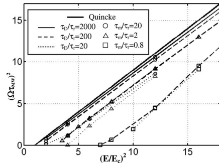
FIG. 5. Squared normalized spin rate vs r=(E_0/E_c)^2 for different values of \tau_m/\tau_r and \tau_D/\tau_r : solid lines: \tau_D/\tau_r=2000 , dashed lines: \tau_D/\tau_r=200 , dotted lines: \tau_D/\tau_r=20 , circles: \tau_m/\tau_r=20 , triangles: \tau_m/\tau_r=2 , squares: \tau_m/\tau_r=0.8 . The thick line corresponds to the predictions of the classical Quincke rotation model.
