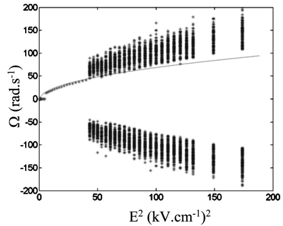
FIG. 5. Bifurcation diagram: For the stationary regime, the angular velocity \Omega is plotted vs the square of the electric field intensity. For the chaotic regime, we have reported the maxima of \Omega verifying |\dot{\Omega}| > \Omega_{\text{st}} . The solid line represents the predicted stationary angular velocity.
