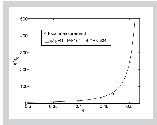
Figure 17: Variation of the relative viscosity deduced from PIV measurements with the particle volume fraction. The measurement has been performed at r = 0.77 R_{out} and the applied torque has been controlled for the bob angular velocity to be approximately 0.4 rpm (Laser position above the bottom of the cup: z = 14 mm. Height of the suspension h = 45 mm).
