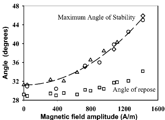
FIG. 9. Measured maximum angle of stability vs rotating magnetic field amplitude for three initial values of the height of the heap. ( \diamond ) 2.75 cm; ( \circ ) 3.2 cm; ( \triangle ) 4.4 cm. Dashed line—best fit of the MAS curve to the relation (16); n_{\text{expt}}=1.95 ; A_{\text{expt}}=1.7 \times 10^{-7} ; ( \blacksquare )—angle of repose vs rotating field intensity.
