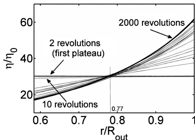
FIG. 6. Long time evolution of the normalized viscosity profile for the \phi=0.444 suspension.
