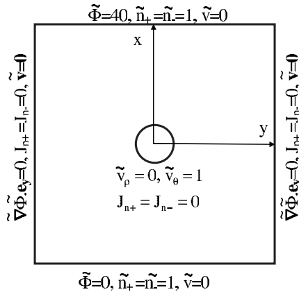
FIG. 3. Boundary conditions for the normalized equations. An insulating cylinder (normalized radius, 1) is placed in a square box (normalized edge length, 40).
