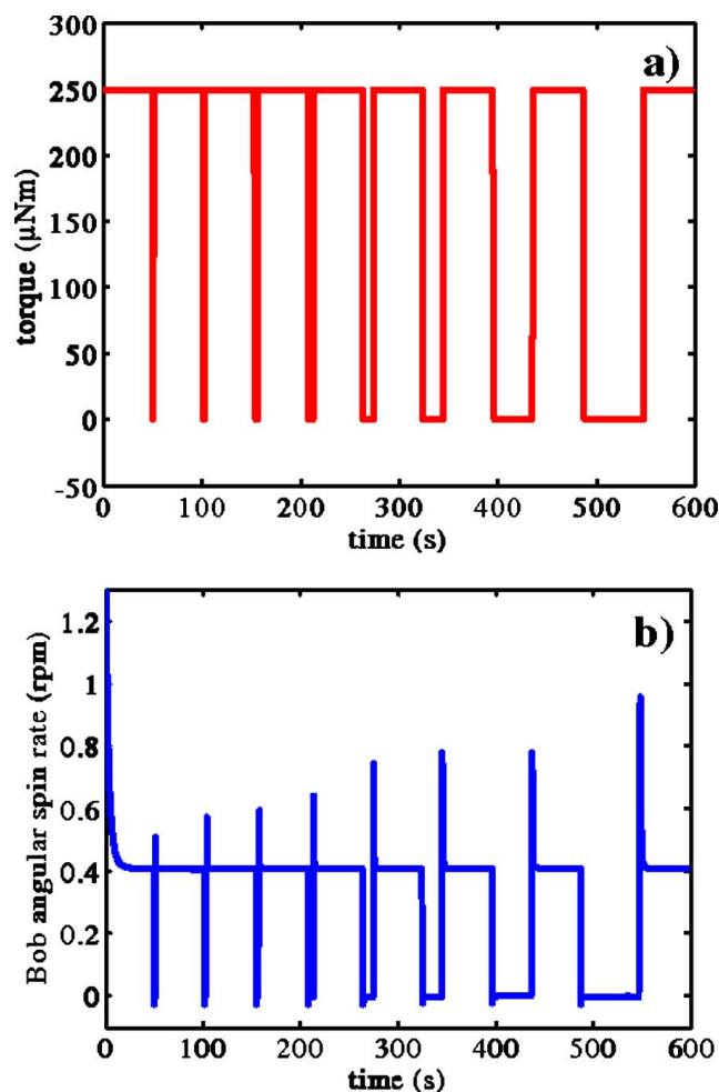
FIG. 14. Sequence of shearing and shear stress break with increasing of the break duration. (a) Applied torque. (b) Bob angular velocity response. The velocity overshoot amplitude increases with the break duration, \phi=0.444 .
