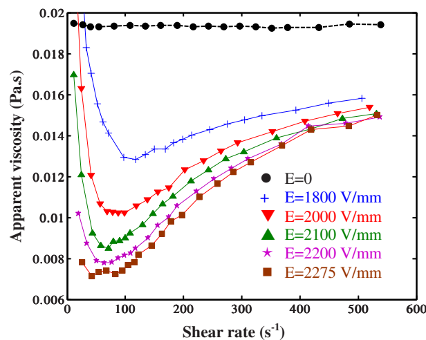
FIG. 10. Variation of the effective viscosity with the shear rate measured with a controlled stress rheometer in Couette geometry for different field intensities.
