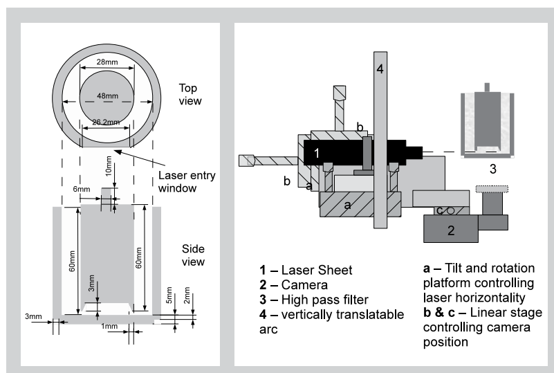
Figure 2 (left above): Schematic drawing of the Couette geometry that is used for the PIV measurements. Both cylinders are made of plexiglas. Their surfaces in contact with the suspension have been roughened to minimize wall slip when the suspension is sheared.
