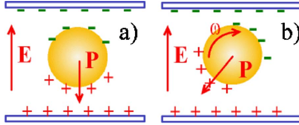
FIG. 1. Representation of the particle dipole, \mathbf{P} , coming from the interfacial charge distribution. If the charge relaxation time is higher in the particle than in the host liquid ( \tau_1 \tau_2 ), \mathbf{P} is anticollinear to the field direction (a). If the E field intensity is high enough, this situation is unstable and the particle rotates either in a clockwise or a counter-clockwise direction. In such a case, the rotation of the particle at constant velocity and the tilt of \mathbf{P} correspond the stationary equilibrium of the system.
