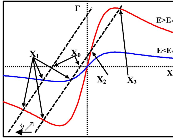
FIG. 3. Variation of the driving electric torque (solid lines) and of the opposite of the viscous resistant torque (dashed lines) exerted on a particle with its angular velocity. The electric torque has been drawn for two intensities of the electric field and the viscous one for two values of the average shear rate in the suspension. Depending both on the values of the field intensity and of the mean shear rate, there exists either one or three solutions for the angular velocity of the particle.
