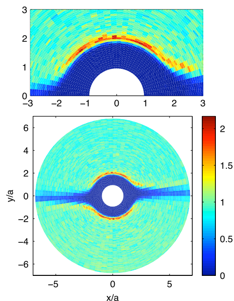
FIG. 3 (color online). Pair distribution function in the plane (\vec{v}, \vec{V}\vec{v}) . \phi = 5\% . The approach quadrants are defined by xy < 0 . Up: magnification of the central region.
