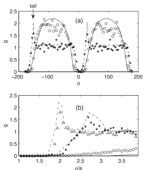
FIG. 7. Experimental (symbols) and computed (lines) PDF. (a) g(\rho, \theta) vs \theta ( ^\circ ) 1.97 < \rho < 2.04 ; ( * ) 2.31 < \rho < 2.38 ; ( - ) 1.93 < \rho < 2.00 ; ( - - ) 2.33 < \rho < 2.40 ; (b) g(\rho, \theta) vs \rho/a ( \circ ) 0 < \theta < 4.5^\circ ; ( * ) 18^\circ < \theta < 22.5^\circ ; ( \Delta ) 85.5^\circ < \theta < 90^\circ ; ( \circ ) 0 < \theta < 4.5^\circ ; ( - - ) 18^\circ < \theta < 22.5^\circ ; ( - \cdot ) 85.5^\circ < \theta < 90^\circ .
