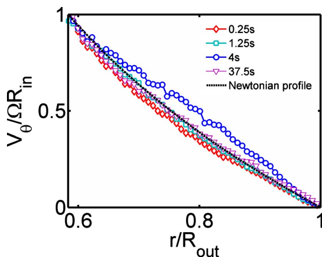
FIG. 7. Transient velocity profiles after shear-reversal (at t=0 the applied torque passes from -250 to +250 \mu\text{N m} ) at different times (0.25, 1.25, 4, and 37.5 s). The dashed line represents the Newtonian profile. \phi=0.444 .
