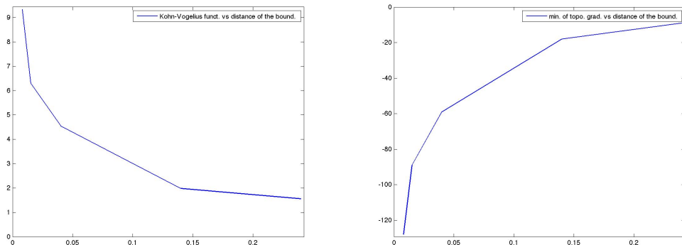
Figure V.7 – The initial Kohn-Vogelius functional and minimum of the topological gradient versus the distance of the obstacle from the exterior boundary d
