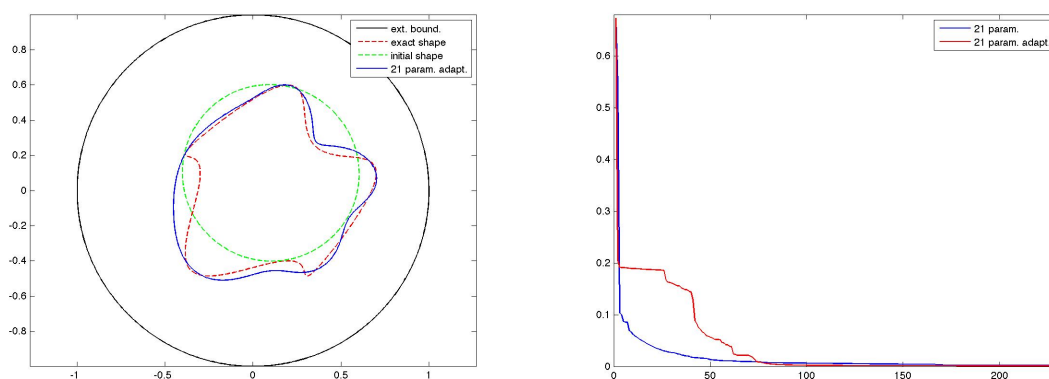
Figure III.3 – Reconstruction of \omega_2^* using the adaptive method with 21 parameters
