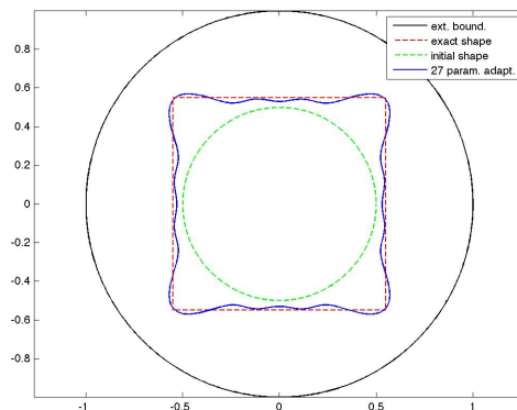
Figure III.4 – Reconstruction of \omega_3^* using the adaptive method with 27 parameters
