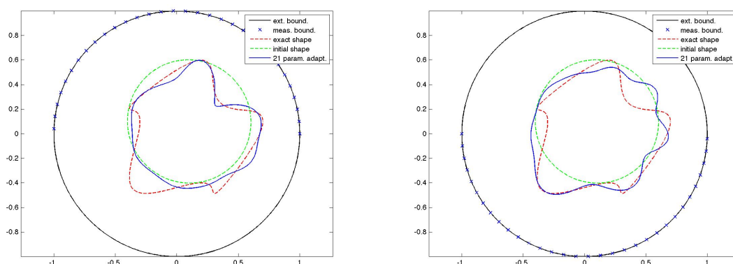
Figure III.6 – Reconstruction of \omega_2^* using the adaptive method with 21 parameters restricting the measurement domain ( O is a half of \partial\Omega )
