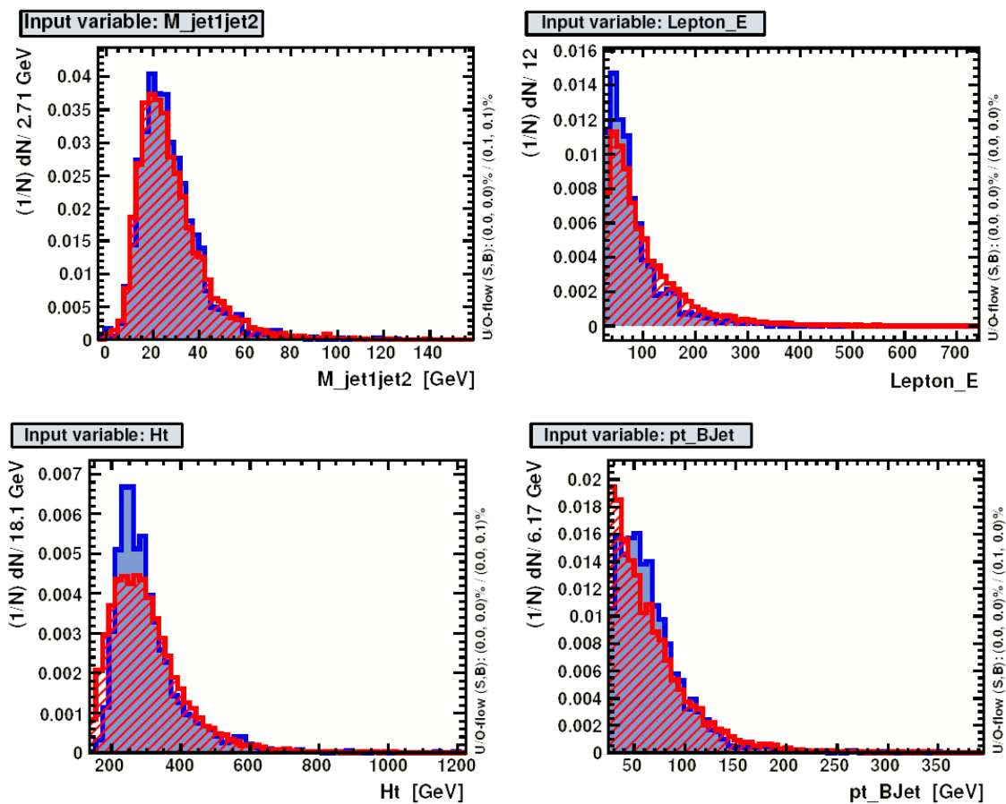
Figure A.3: Normalized distribution of the discriminating variables used as input of the boosted decision tree for signal (blue) and background (red) for 3-jets events.
