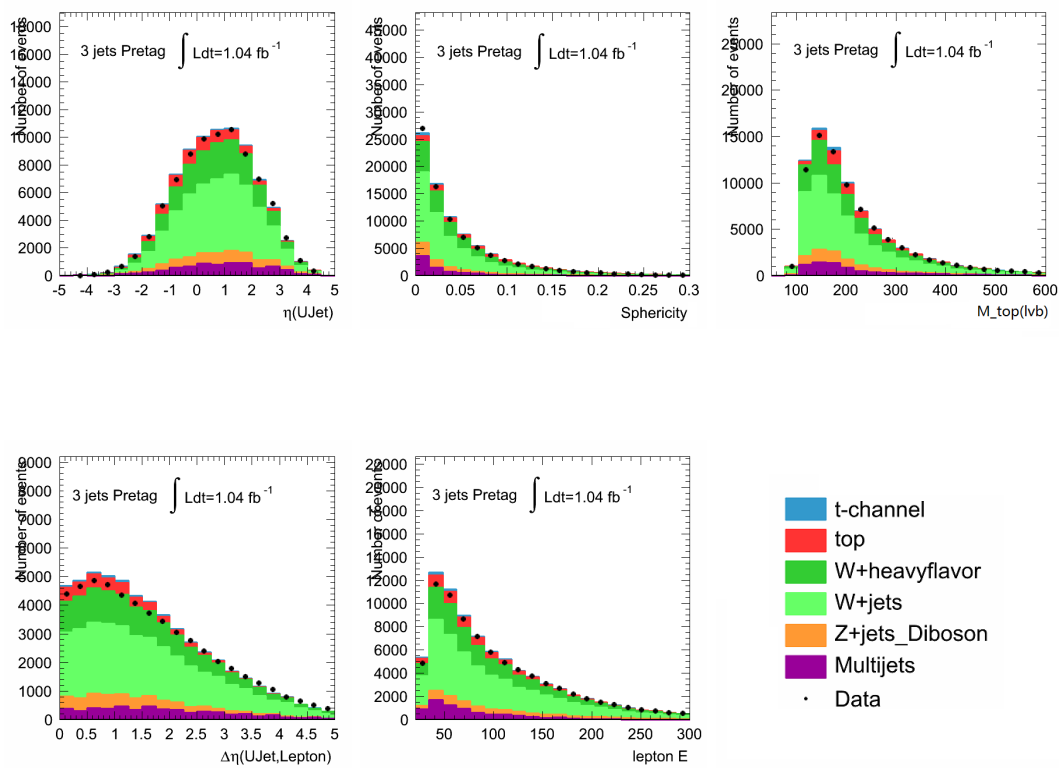
Figure 6.11: Most discriminant variables used as input of the BDT for the 3-jet pretag sample (electron and muon samples combined).
