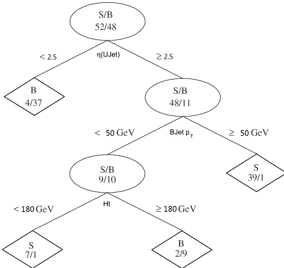
Figure 6.1: An illustration of a decision tree.
