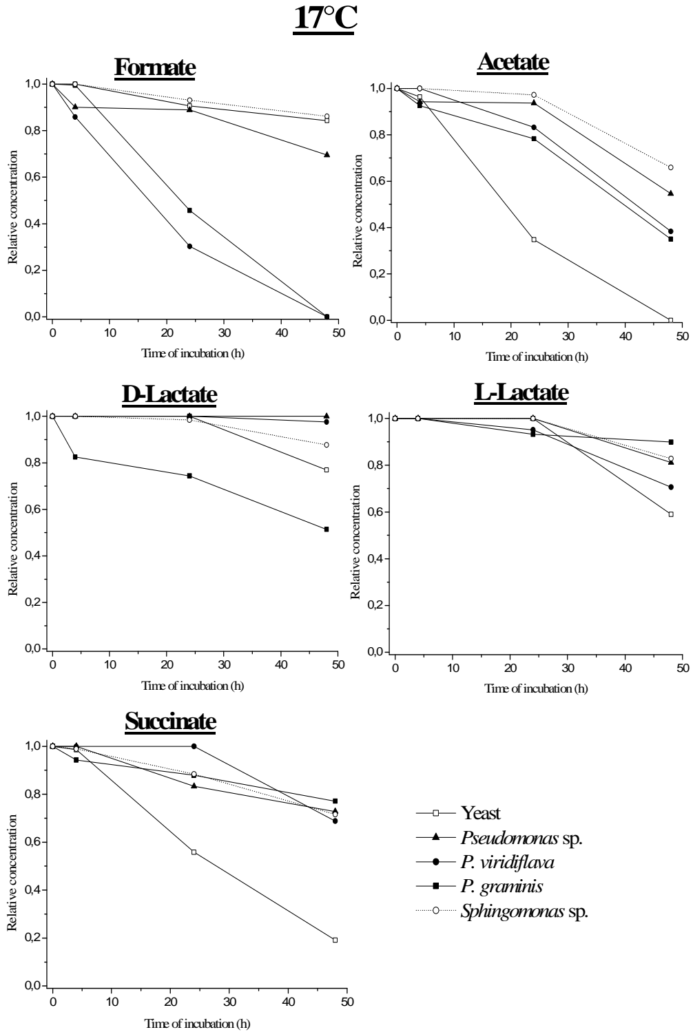
Figure 3: Biodegradations at 17°C of formate, acetate, L- and D-lactate and succinate by the five strains.
