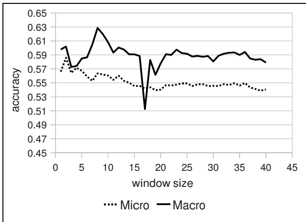
Figure 9.3: Micro and macro accuracy for the first approach (training on Chinese texts)
