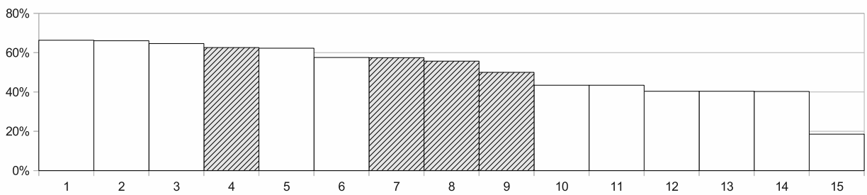
Figure 10.3: Systems performance and ranking on the 3-class track on books (top), movies (middle), and cameras (bottom) collections. Our systems are highlighted
