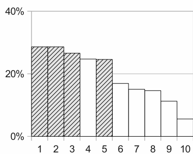
Figure 10.4: Systems performance and ranking on the 5-class track on books (top), movies (middle), and cameras (bottom) collections. Our systems are highlighted
