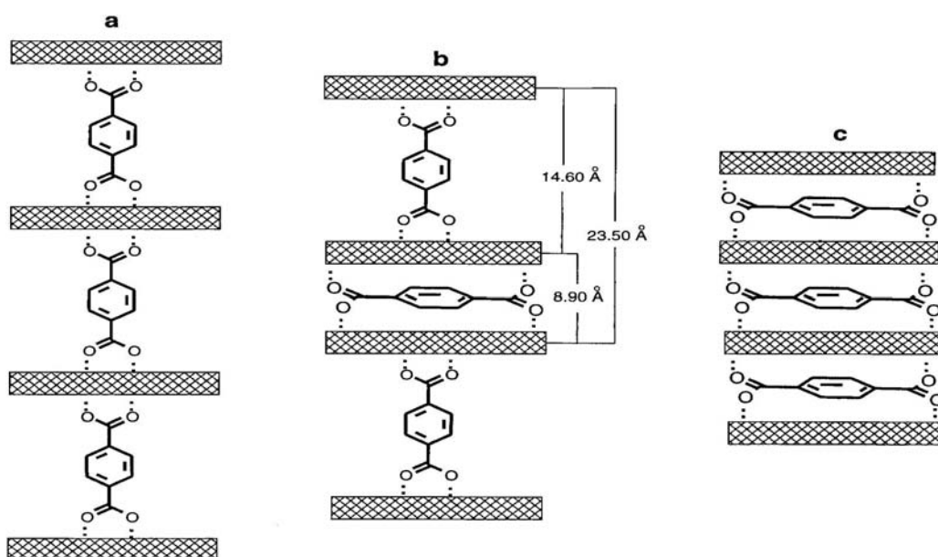
Figure 1-35: Proposed model for structural changes occurring during the heat treatment and loss of the interlayer water of Mg_2Al -Terephthalate at (a) 25 °C, (b) 100 °C and (c) 200 °C. See ref. 208.
