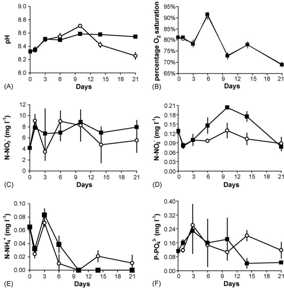
Fig. 1. Evolution of pH values (A), dissolved oxygen (B), and N-NO 3 - (C), N-NO 2 - (D), N-NH 4 + (E) and P-PO 4 3- (F) concentrations in control (○) and treated microcosms (■). Data are presented as means ± S.D. calculated from the three replicate microcosms.
