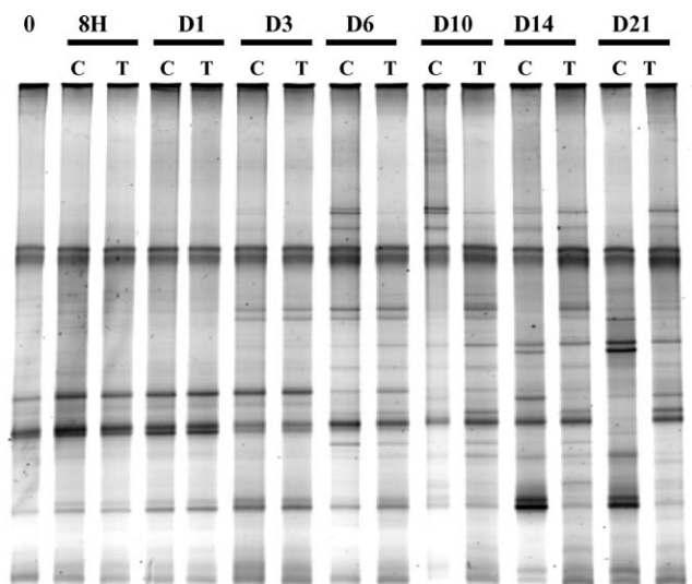
Fig. 8. Average evolution of temporal temperature gradient gel electrophoresis profiles for PCR-amplified 16S rDNA from the V6 to V8 regions in control (C) and treated (T) microcosms at day 0 (0), 8 h (8H) and from day 1 (D1) to day 21 (D21).
