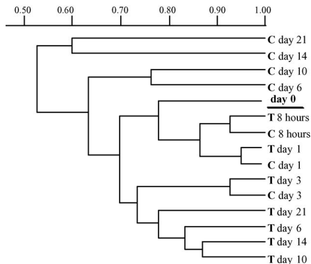
Fig. 9. UPGMA cluster analysis of DICE distance matrix calculated from TTGE banding patterns (based on presence/absence and band weighting).
