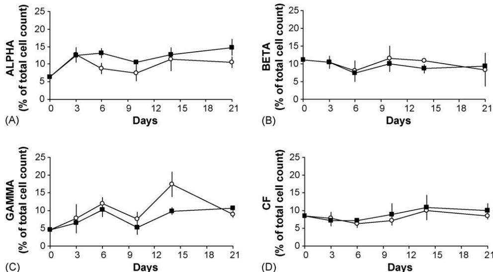
Fig. 7. Average evolution ( \pm S.D.) of relative abundance of the main phylogenetic groups determined by FISH using ALF1b (A), BET42a (B), GAM42a (C) and CF319a (D) in control (○) and treated (■) microcosms.
