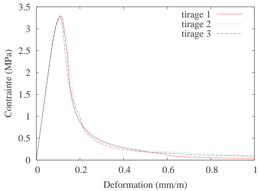
(a) Tension
