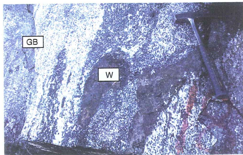
GB=gabbro W=wehrlite
