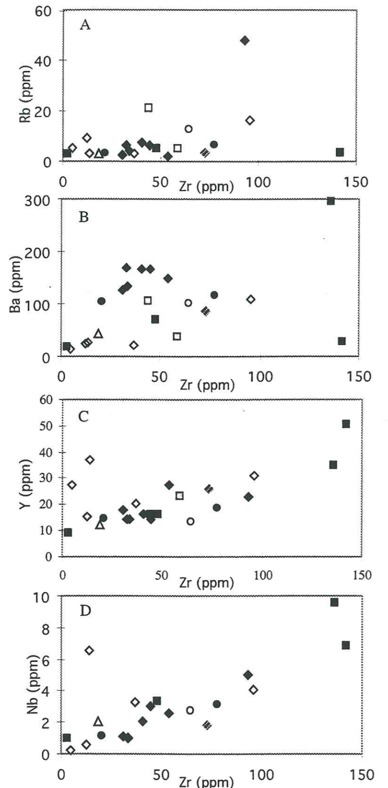
Group-1 metavolcanic rocks ◇ N-Pattan □ N-Kamila Group-2 metaplutonic rocks -coarse-grained metagabbro/metadiorite ◆ N-Pattan ■ N-Kamila ● Swat Valley -sheared metagabbro/metadiorite ◇ N-Pattan ○ Swat Valley -doleritic dyke △ Swat Valley
