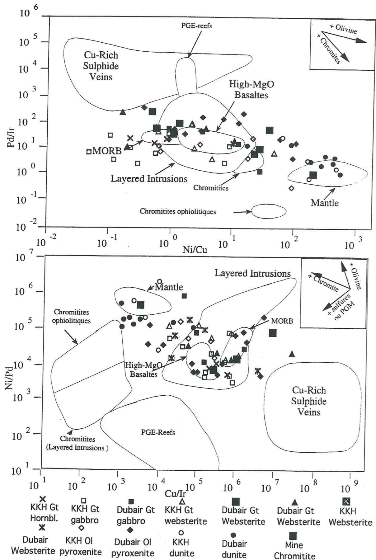
Figure 108. Metal ratio diagrammes of Pd/Ir versus Ni/Cu and Ni/Pd versus Cu/Ir for the Jijal Complex. Fields boundaries for mantle, high-MgO basalt, layered intrusions, PGE-reef, Cu-rich sulphides, chromitite ophiolites, MORB, and mineral-control vectors, are taken from Barnes et al. (1988); Barnes (1990).
