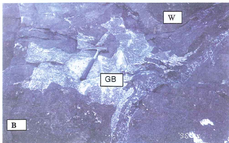
W = Wehrlite GB = Gabbro
