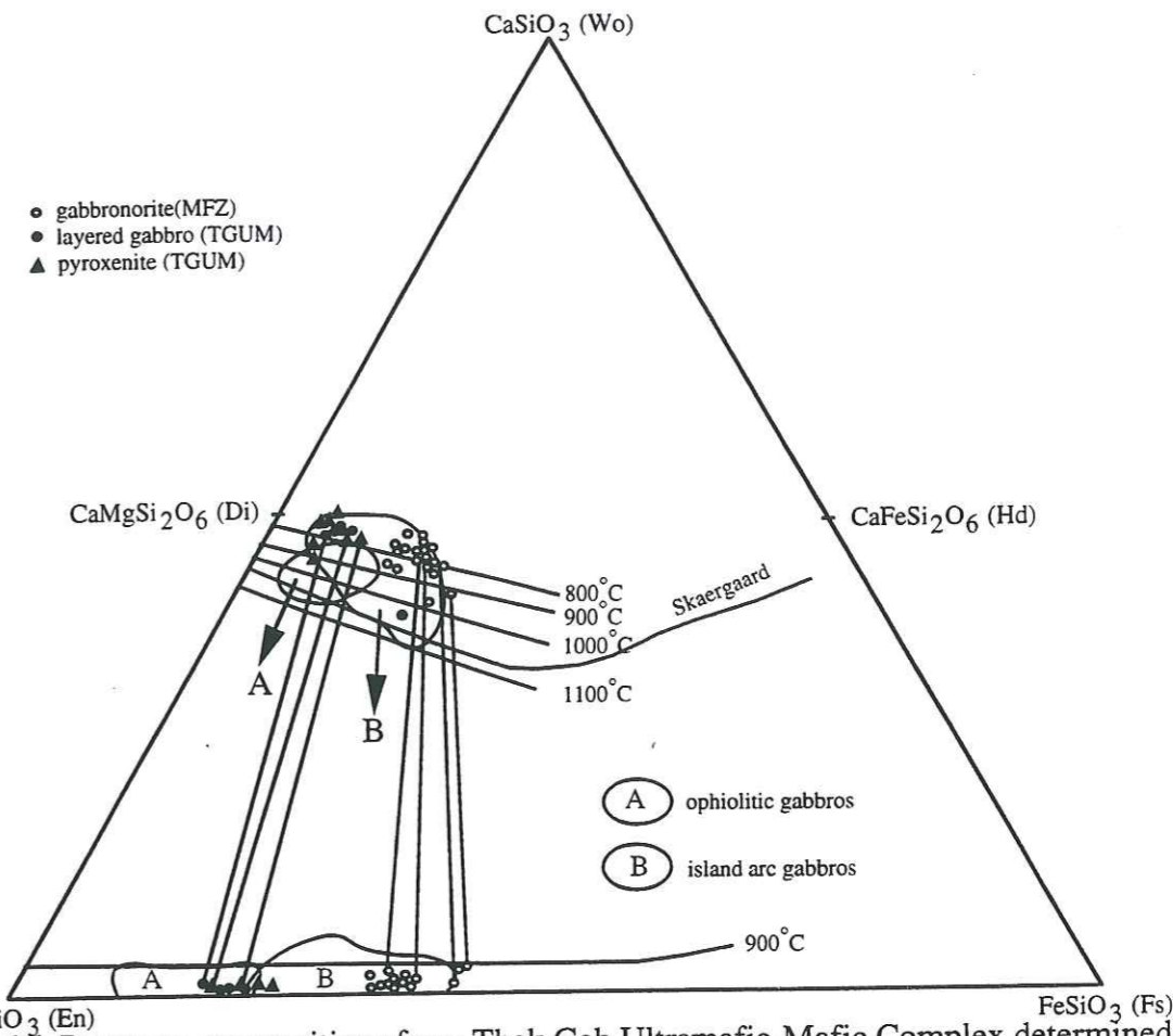
Figure 36. Pyroxene compositions from Thak Gah Ultramafic-Mafic Complex determined by electron microprobe. Compositional fields of island-arc gabbros (Arculus & Wills, 1980; Meijer & Reagan, 1981) and ophiolitic gabbros (Coleman, 1977) are also indicated. The lines connect coexisting pyroxenes. Temperature estimates from Ross and Huebner (1975). Composition des pyroxènes du Complexe mafique-ultramafique de Thak Gah mesurée par microsonde électronique. Les lignes relient les pyroxènes coexistants
