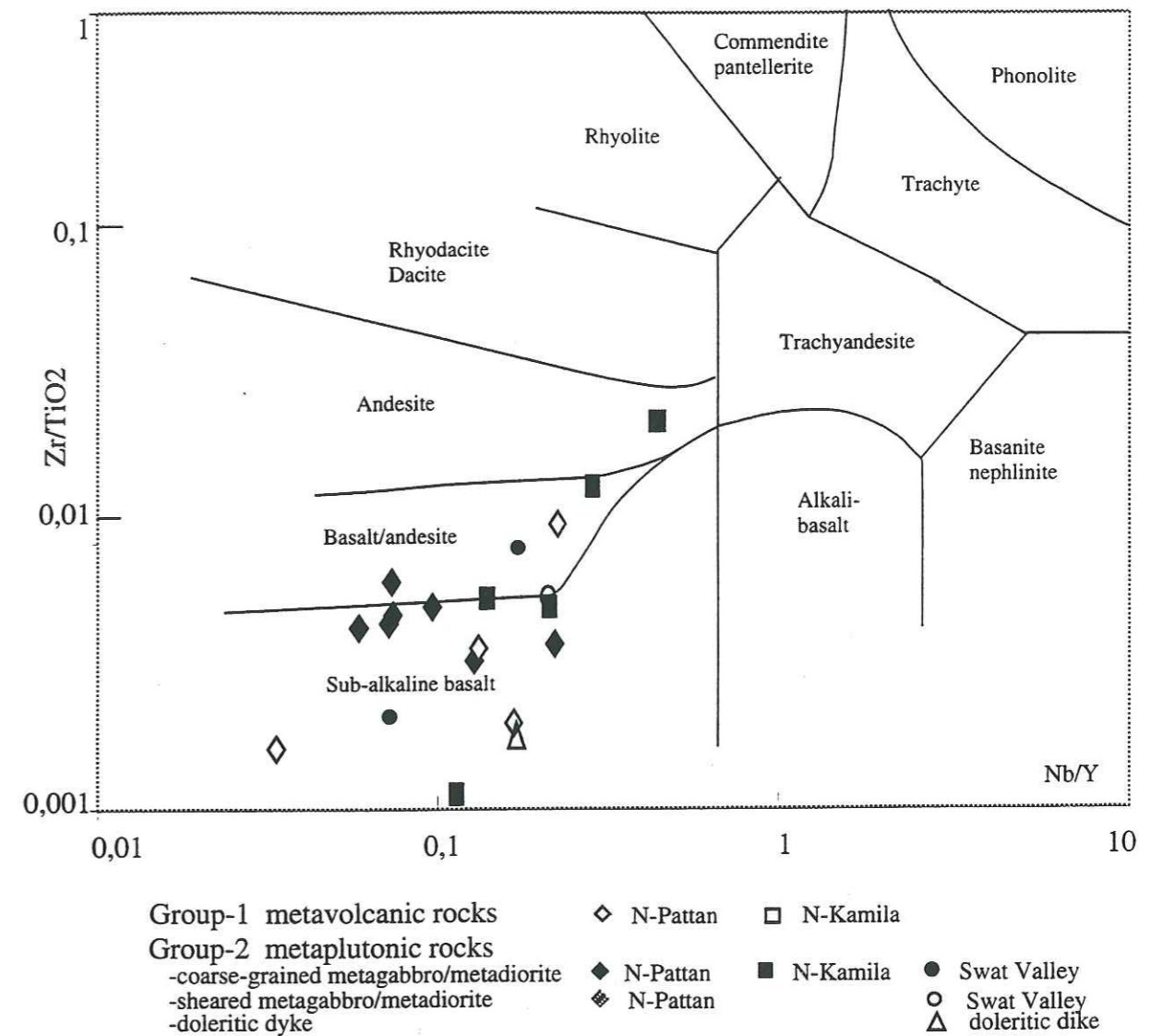
Figure 11. Zr/TiO 2 versus Nb/Y plot (Winchester & Floyd, 1977) for the different facies of the Kamila Amphibolites.
