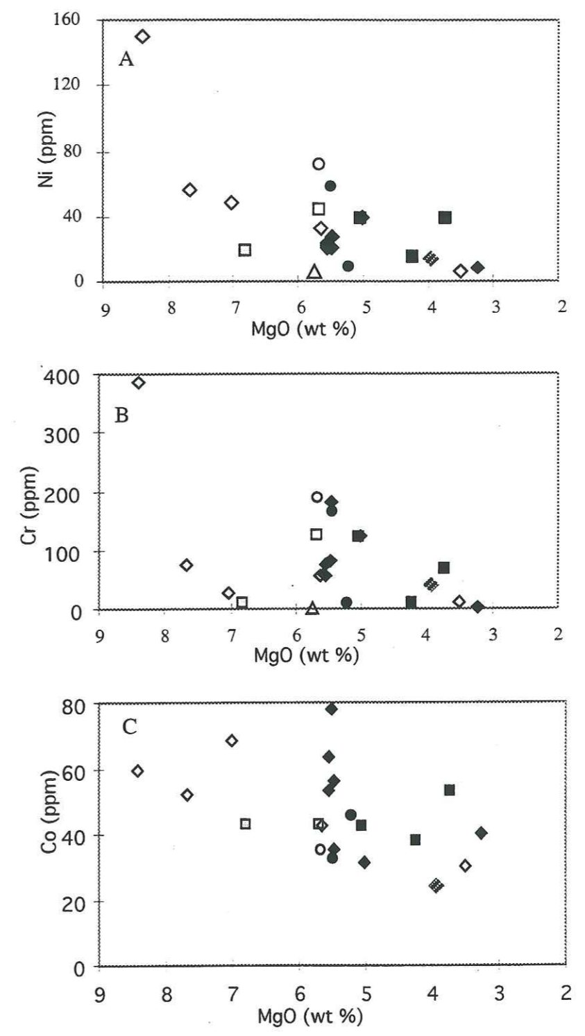
Group-1 metavolcanic rocks ◇ N-Pattan □ N-Kamila Group-2 metaplutonic rocks -coarse-grained metagabbro/metadiorite ◆ N-Pattan ■ N-Kamila ● Swat Valley -sheared metagabbro/metadiorite ◇ N-Pattan ○ Swat Valley -doleritic dyke △ Swat Valley
