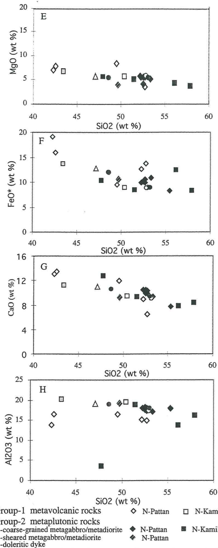
Figure 8. Harker variation diagrams for major elements in different facies of the Kamila Amphibolites.
