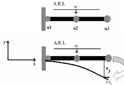
Figure II.3.3: cantilever beam.
