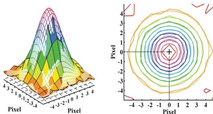
Fig. A single imaged fluorophore can be modelled by a two-dimensional Gaussian to determine its position with nanometer accuracy. The three-dimensional peak to the left shows the recorded intensity for each pixel as a coloured surface. A corresponding contour map is shown to the right (Walter et al., 2008).
