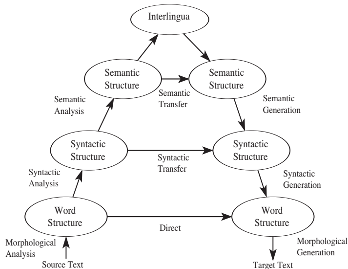
Figure 2.2: Analysis performed in machine translation pyramid
