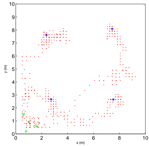
Figure 4.11: Four robots with a maximum monitoring distance r = 3.5m in a convex environment. The green points show the initial positions of the robots, the final ones are in blue, in red the trajectories. The solution reproduces the centroidal Voronoi solution, where the robots' positions are the generator of the partition.
