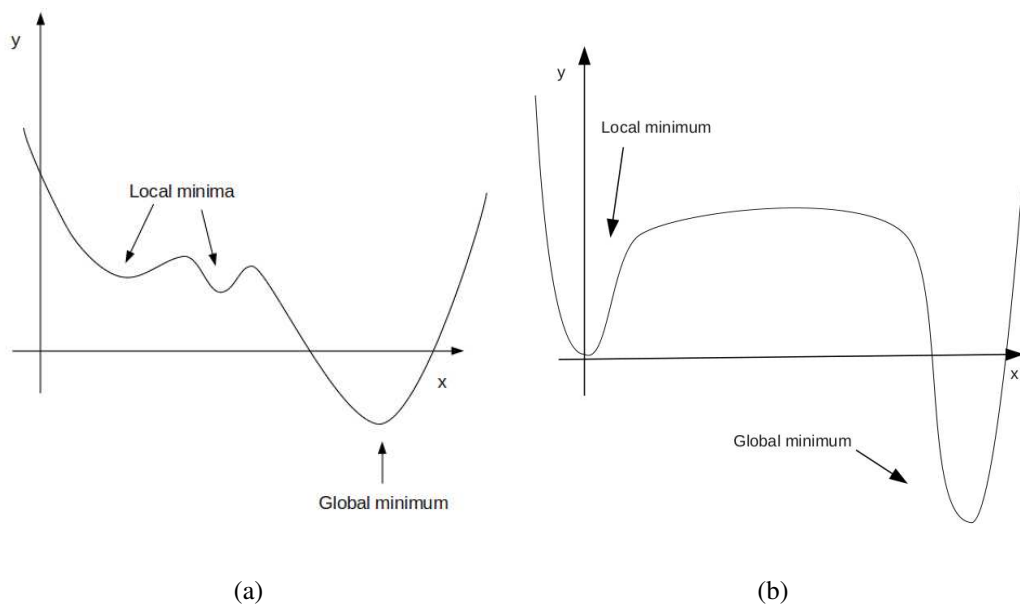
Figure 2.1: Two different simple examples of local minima: in (a) two local minima are present but their dimension is such that the global minimum is easy to find. In (b) there is only one local minimum but a higher barrier, hard to overcome, divides it from the global minimum. In this case the initial position is crucial for the final result.
