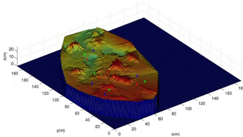
Figure 6.12: Final configurations of three robot teams starting from different initial positions for the Birnensdorf area.
