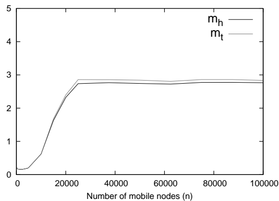
Figure 8.9: Verification of number of hops and transmission attempts with plots of m_h and m_t .
