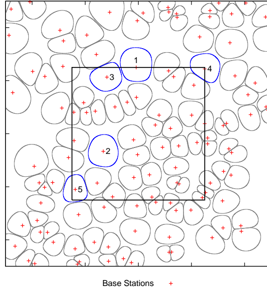
Figure 5.4: 5 base stations are added to the area of interest \mathcal{A}_R using Heuristic 2 . The number indicates the order of addition to the network. \beta = 1.0 and \alpha = 4.0 .
