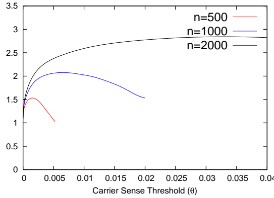
Figure 7.4: Optimization of the throughput capacity \zeta(n, 20.0, 4.0) (packets per slot) with CSMA based scheme in network with uniform distribution of nodes under no fading . \beta = 20.0 and \alpha = 4.0 .
