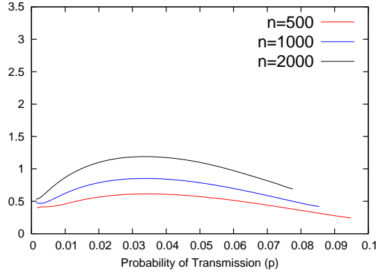
Figure 7.2: Optimization of the throughput capacity \zeta(n, 20.0, 4.0) (packets per slot) with slotted ALOHA scheme in network with uniform distribution of nodes under no fading . \beta = 20.0 and \alpha = 4.0 .
