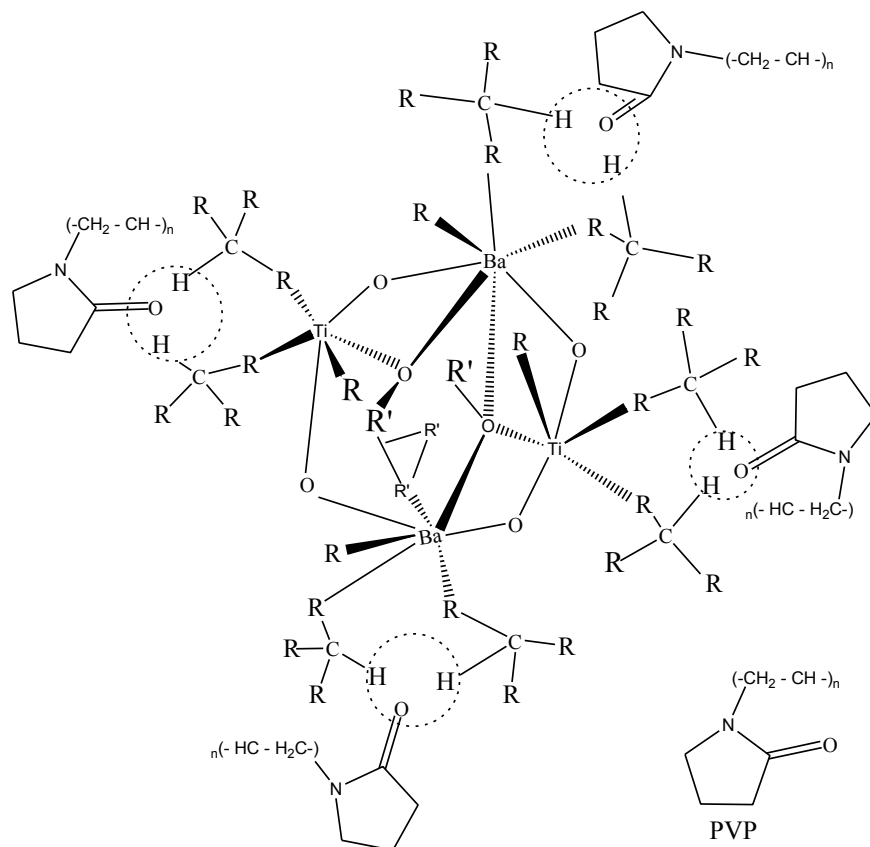
Figure 5-34. Structure of intermediate alkoxide complexes of barium and titanium in presence of PVP.
