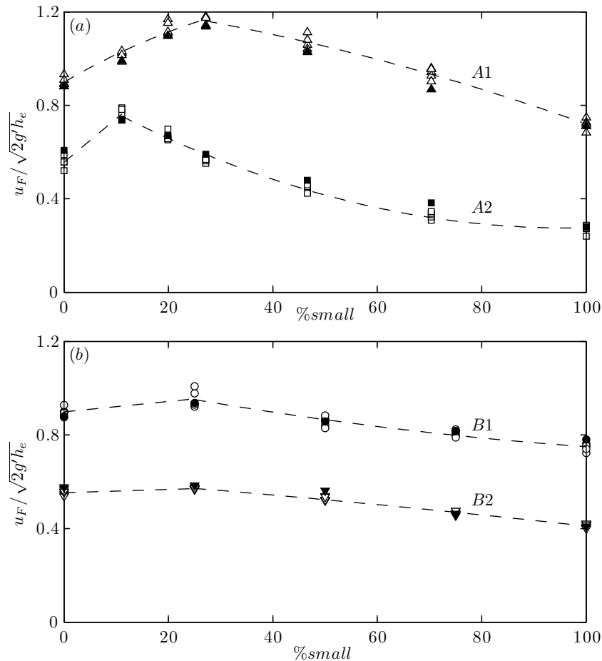
FIGURE 5.12. Froude number Fr = u_F / \sqrt{2g'h_e} as a function of the initial volume fraction of small grains for sets A1 (in air, \Delta ) and A2 (in water, \square ) (a), and B1 (in air, \circ ) and B2 (in water, \nabla ) (b) of table 3.2. White marks are experimental measurements with h_o/x_o=2,3,4,6,8 ; and black marks are simulation results with h_o/x_o=6 and \sigma=1.4 . The experimental tendency is represented by the dashed line.
