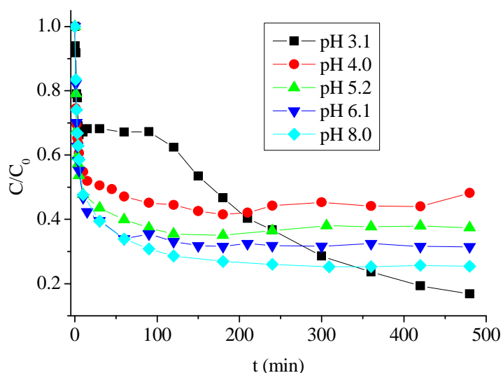
Figure IV-B-8 Effect of pH on the degradation of E2 ( [\text{Fe(III)-EDDS}] = 1 \times 10^{-4} \text{ M} , [\text{E2}] = 5 \mu\text{M} ).
