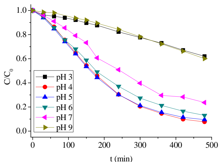
Figure IV-F-13 Influence of pH on the photodegradation of E2 in aqueous solutions containing Goethite in the presence of EDDS. The experimental conditions were as follows: [E2] = 5 \mu\text{M} , [Goethite] = 0.05 \text{g L}^{-1} , [EDDS] = 250 \mu\text{M} , irradiation time 8 hours.
