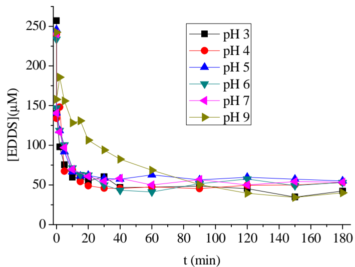
Figure IV-D-12 Concentration of EDDS during the irradiation ( [\text{KSF}] = 1 \text{ g L}^{-1} , [\text{E2}] = 5 \text{ }\mu\text{M} , [\text{EDDS}] = 250 \text{ }\mu\text{M} , irradiation time 3 h).
