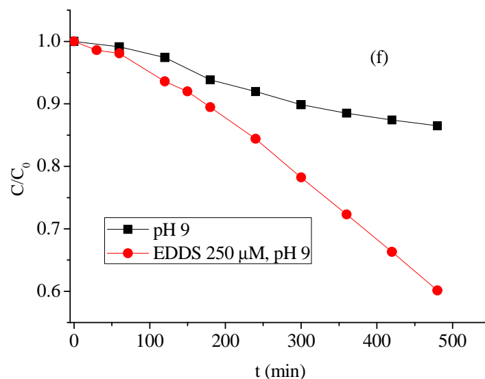
Figure IV-F-17 Comparison of the effect of pH on the photodegradation of E2 with EDDS in Goethite suspensions with or without EDDS. (a): pH 3; (b) pH 4; (c) pH 5; (d) pH 6; (e) pH 7; (f) pH 9 ([E2] = 5 μM, [Goethite] = 0.05 g L -1 , [EDDS] = 250 μM, irradiation time 8 hours).
