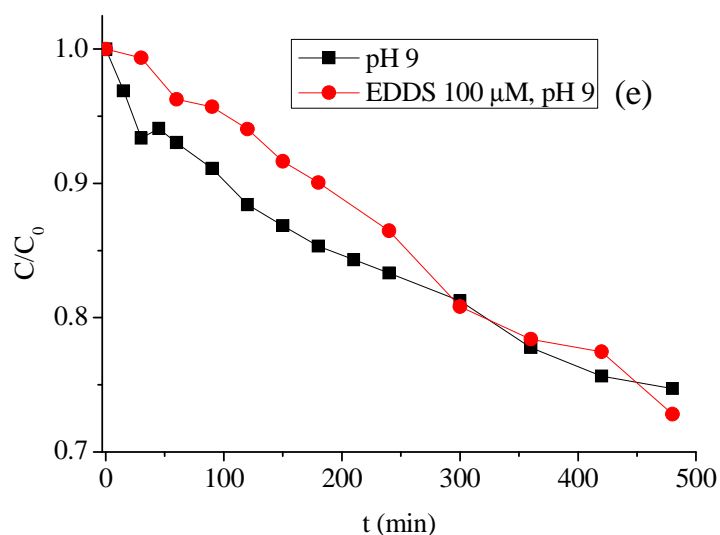
Figure IV-E-15 Comparison of the effect of pH on the photodegradation of E2 with or without EDSS in NM suspensions. (a): pH 3; (b) pH 4; (c) pH 5; (d) pH 7; (e) pH 9 ([EDDS] = 100 \mu\text{M} , [E2] = 5 \mu\text{M} , [NM] = 6 \text{g L}^{-1} ).
