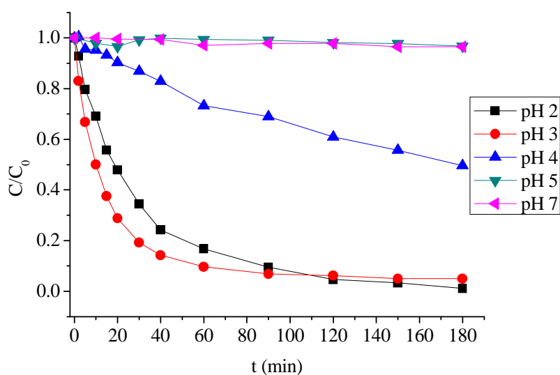
Figure IV-D-5 Influence of pH on the photodegradation of E2 in aqueous solutions containing KSF. The experimental conditions were as follows: [\text{E2}] = 5 \mu\text{M} , [\text{KSF}] = 1 \text{ g L}^{-1} , irradiation time 3 h.
