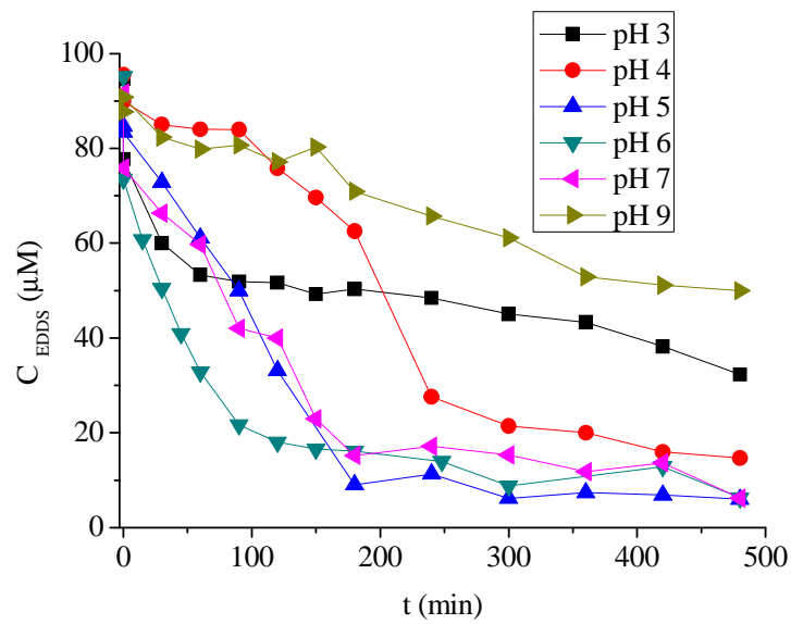
Figure IV-E-14 Change of EDDS concentration during the photodegradation of E2 under the different pHs ([EDDS] = 100 μM, [E2] = 5 μM, [NM] = 6 g L -1 )
