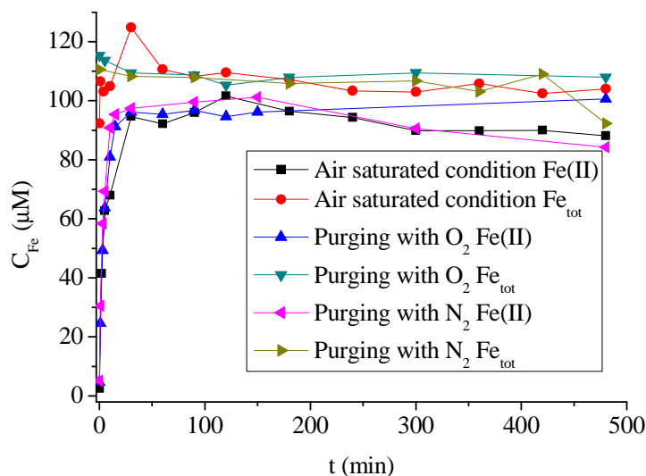
Figure IV-B-12 Concentration of Fe(II) and Fe(tot) during the irradiation ([Fe(III)-EDDS] = 10 -4 M, [E2] = 5 μM)
