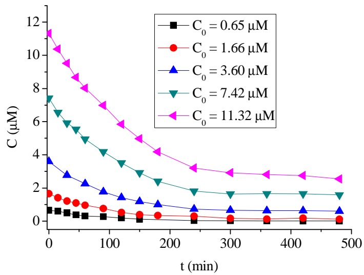
Figure IV-E-18 Influence of initial E2 concentration on the photodegradation of E2 in NM solutions in the presence of EDDS. The experimental conditions were as follows: [NM] = 6 g L -1 , [EDDS] = 250 µM, pH = 5.0, irradiation time 8 h.
