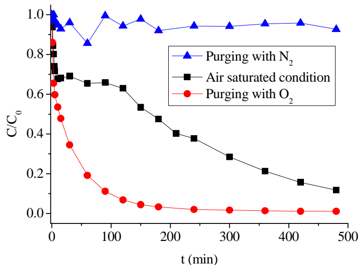
Figure IV-B-11 Effect of oxygen on the degradation of E2 ([E2] = 5 μM, [Fe(III)-EDDS] = 1×10 -4 M, pH = 3.0).
