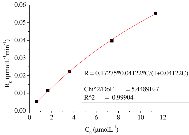
Figure IV-E-19 Plots of Ro versus Co for E2 degradation in the NM suspensions in the presence of EDDS
