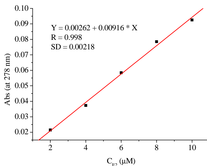
Figure IV-A-2 Molar absorption coefficients at 278 nm.
