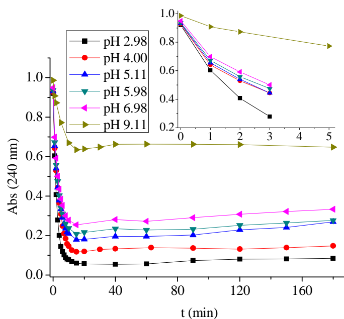
Figure IV-A-10 The A_{\lambda=240\text{ nm}} (Fe(III)-EDDS) at the different time under the different pH
