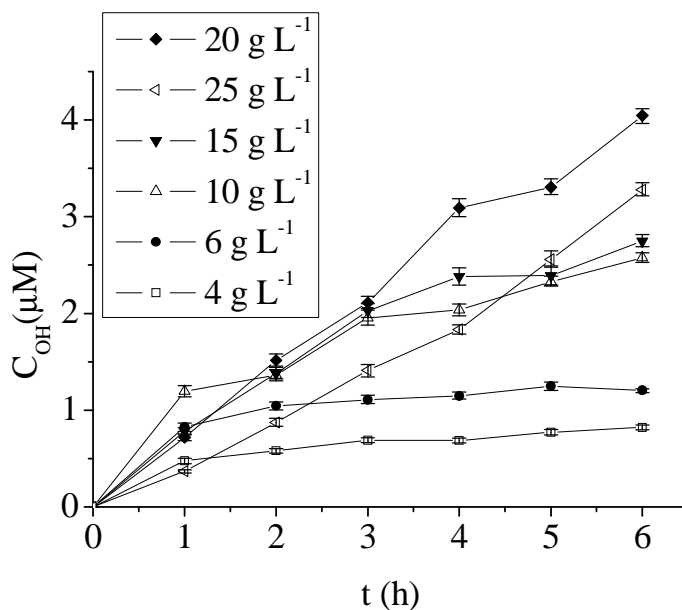
Figure IV-C -3 Influence of clay concentration on the hydroxyl radicals formation in aqueous suspensions containing Montmorillonite (4.0 to 25.0 \text{g L}^{-1} ). The experimental conditions were as follows: [benzene] = 7 mM, irradiation time 6 hours, pH = 9.8 (without adjusting).
