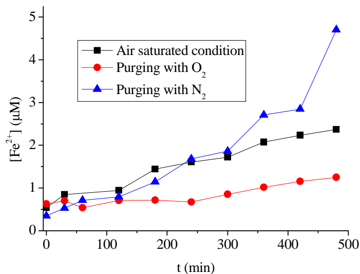
Figure IV-F-20 Concentration of iron during the irradiation ( [\text{Goethite}] = 0.05 \text{ g L}^{-1} , [\text{EDDS}] = 250 \text{ }\mu\text{M} , [\text{E2}] = 5 \text{ }\mu\text{M} , pH 4.0, irradiation time 8 hours).
