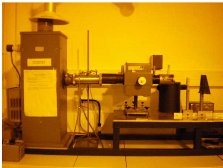
Figure III-C-1 Picture of the monochromatic irradiation device
