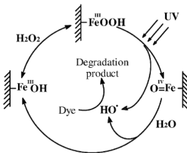
Scheme II-A-2 Fe cycling in the Goethite/ H_2O_2 /UV system(He et al. , 2002).
