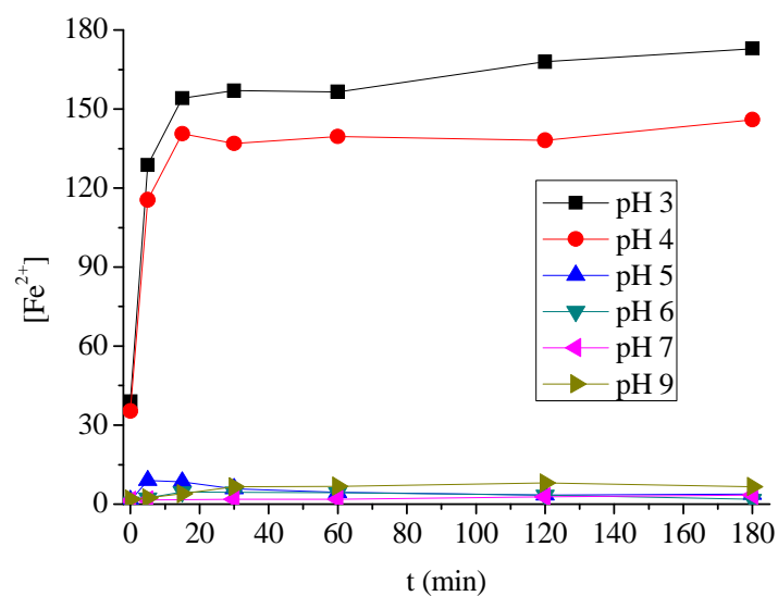
Figure IV-D-11 Concentration of Fe(II) during the irradiation ( [\text{KSF}] = 1 \text{ g L}^{-1} , [\text{E2}] = 5 \text{ }\mu\text{M} , [\text{EDDS}] = 250 \text{ }\mu\text{M} , irradiation time 3 h).
