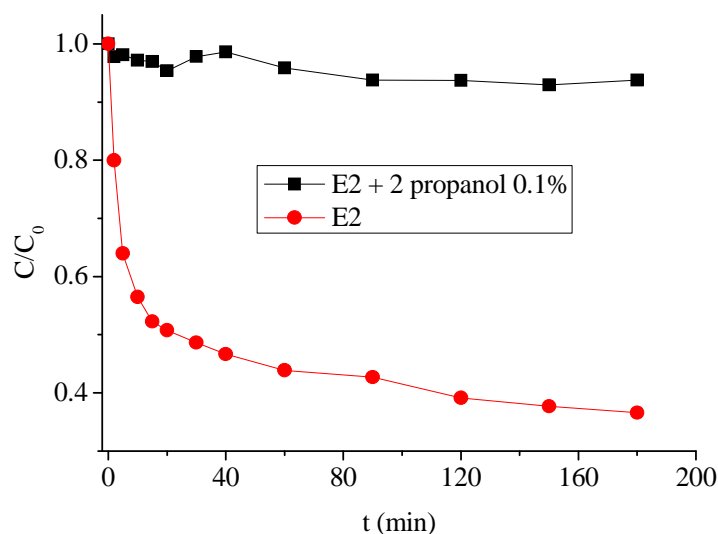
Figure IV-D-21 Influence of 2-propanol on the photodegradation of E2 in KSF solutions in the presence of EDDS. The experimental conditions were as follows: [KSF] = 1 g L -1 , [EDDS] = 250 μM, [E2] = 5 μM, pH 6.0, irradiation time 3 h.
