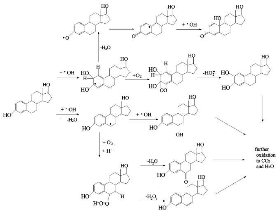
Scheme II-C-1 Simplified mechanism of E2 photodegradation (Zhao et al. , 2008)
