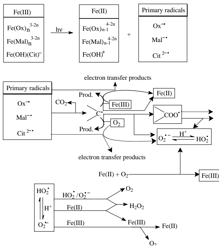
Figure II-B-5 Reaction scheme for the photolysis of Fe(III)-polycarboxylate complexes (Zhang, 2009)
