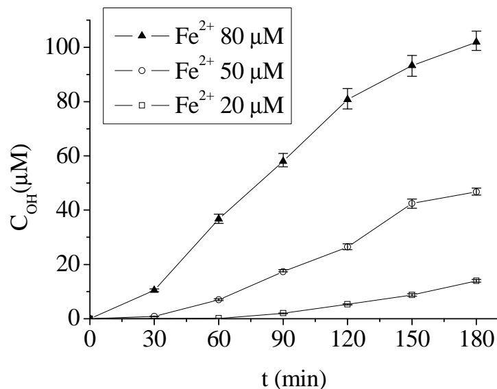
Figure IV-C-6 Influence of the concentration of Fe 2+ on the hydroxyl radical formation in aqueous solutions containing Fe 2+ at different concentrations 20, 50 and 80 μM. The experimental conditions were as follows: [benzene] = 7 mM, irradiation time 3 hours, pH =3.0.
