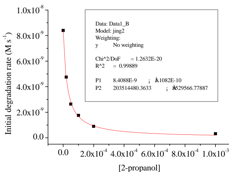
Figure IV-B-4 Initial degradation rate of 232 μM EDDS upon monochromatic irradiation ( \lambda = 313 nm) of 0.1 M \text{NO}_3^- ( \text{NaNO}_3 ), at pH 3, as a function of the initial concentration of 2-propanol. The experimental data were fitted with equation (5) to get k_{\text{EDDS}, \bullet\text{OH}} = 2.0 \times 10^8 \text{ M}^{-1}\text{s}^{-1} , R_{\bullet\text{OH}} = 8.4 \times 10^{-9} \text{ M s}^{-1} .
