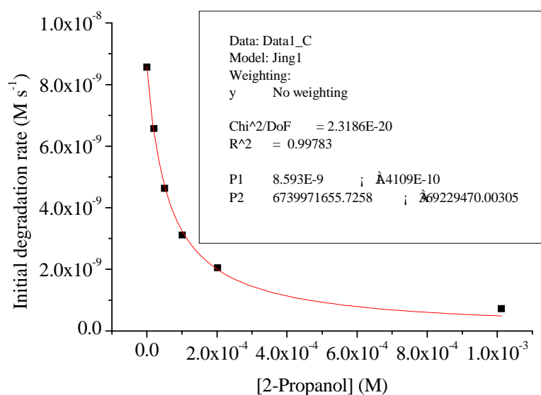
Figure IV-B-3 Initial degradation rate of 17.2 μM E2 upon monochromatic irradiation ( \lambda = 313 nm) of 0.1 M \text{NO}_3^- ( \text{NaNO}_3 ), at pH 3, as a function of the initial concentration of 2-propanol. The experimental data were fitted with equation (5) to get k_{\text{E2}, \bullet\text{OH}} = 6.7 \times 10^9 \text{ M}^{-1}\text{s}^{-1} , R_{\bullet\text{OH}} = 8.6 \times 10^{-9} \text{ M s}^{-1} .
