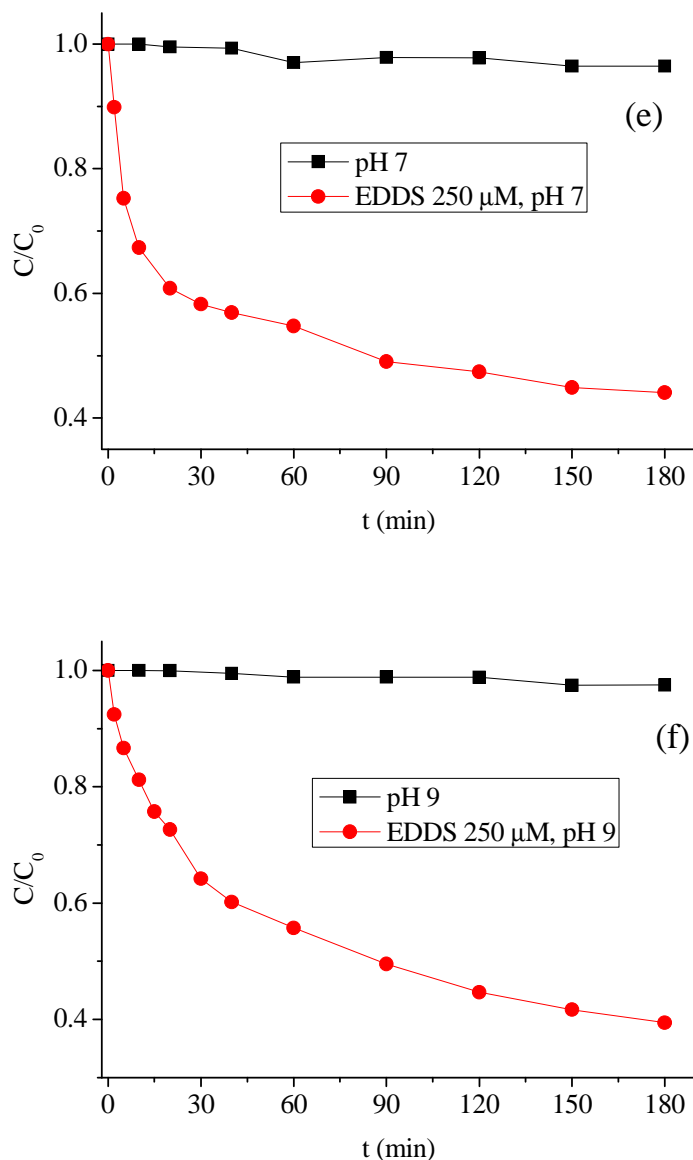
Figure IV-D-13 Comparison of the photodegradation of E2 with and without EDDS at different pHs. (a): pH 3; (b) pH 4; (c) pH 5; (d) pH 6; (e) pH 7; (f) pH 9 ( [\text{KSF}] = 1 \text{ g L}^{-1} , [\text{E2}] = 5 \mu\text{M} , [\text{EDDS}] = 250 \mu\text{M} , irradiation time 3 h).
