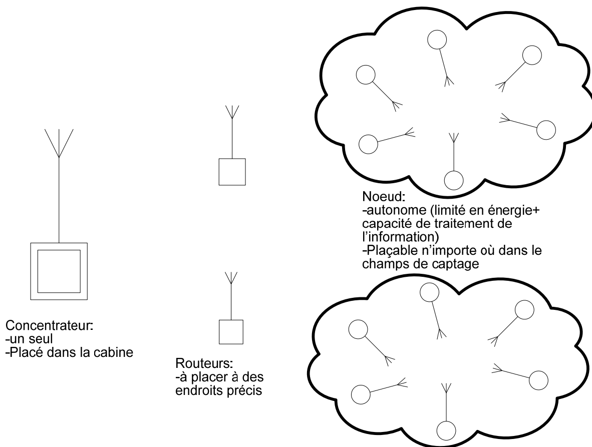
Figure 1. 1 Architecture des RCSFs
