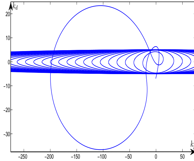
Figure 8.9: Corresponding crossing curves for (8.22).
