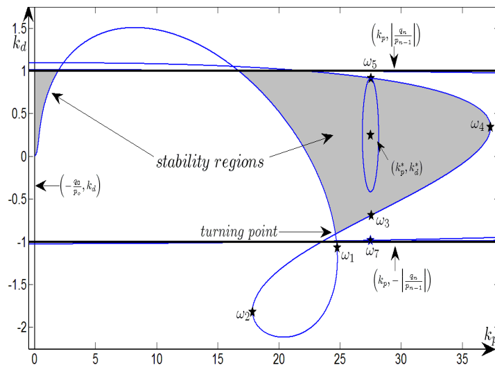
Figure 8.15: Multi-stability region for (8.24).
