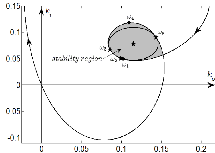
Figure 8.8: The stability crossing curves for the dynamic system (8.10), the boundary of the stability region (shaded region) in the (k_p, k_i) parameters space and the maximum parameter deviation without losing stability.
