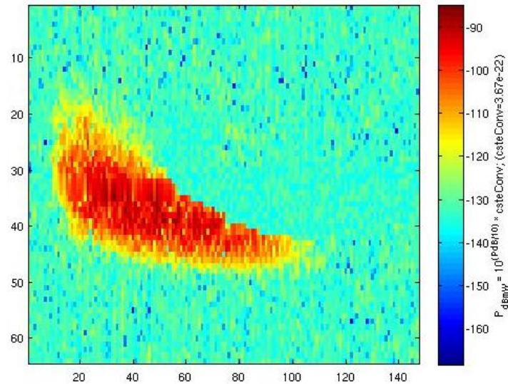
Figure V.15. Radargram of gate 2607 m with power values expressed in dBmW, using the radar conversion constant C_{conv} . Axis units refer to the pixels counted from the top left corner of the radargram.
