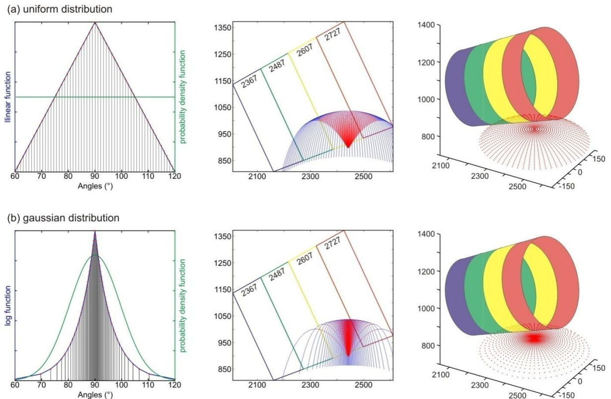
Figure IV.6. Simulated eruptive jets, with respectively linear (a) and Gaussian (b) distributions of ejection angles in the vertical (xoy) plane (middle panel). In both cases, the distribution is then rotated 180° around the (vertical) jet axis to simulate 3D dynamics.
