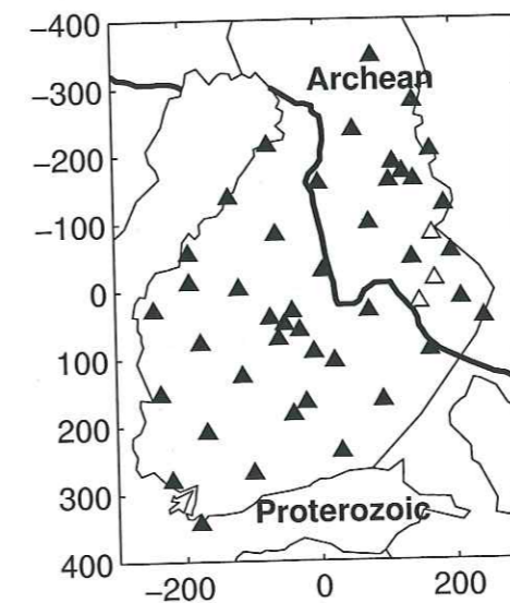
FIG. 5.1 – Map of the broadband stations of the SVEKALAPKO array (CMG3 and STS2, cut-off frequency 90-100 s: filled triangles, CMG40, cut-off frequency 40-60 s: open triangles). The thick line gives the boundary between the Archean Karelian province in the north-east and the Proterozoic Svecofennian domain in the south-west.
