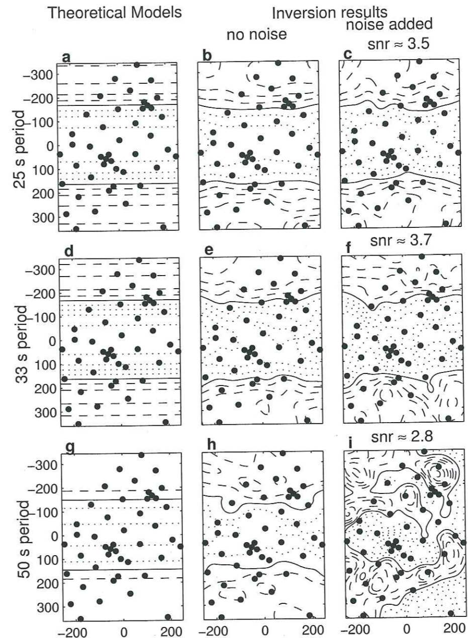
FIG. 3.10 – Inversion of time delays measured on IBEM synthetic seismograms. On each plot the contours are every 0.03 \text{ km.s}^{-1} , dotted lines are for lower velocities, dashed line for larger velocities. a) b) c) model for 25 s period, solid line for 4.02 \text{ km.s}^{-1} . d) e) f) 33 s period, solid line for 4.23 \text{ km.s}^{-1} . g) h) i) 50 s period, solid line for 4.44 \text{ km.s}^{-1} . a) d) g) theoretical local phase velocities. b) e) h) models obtained from inversion of signals without noise. c) f) i) models obtained from inversion of the noisy signals; snr: signal to noise ratio. Black dots give the station locations.
