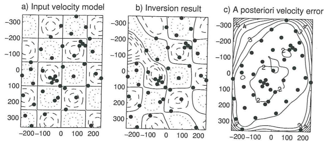
FIG. 3.7 – Sensitivity test. a) true velocity model used to compute the arrival times. b) velocity model obtained after 2 iterations of the inversion. Contours are every 0.04 \text{ km.s}^{-1} , solid line for 4.1 \text{ km.s}^{-1} , dotted lines for lower velocities, dashed line for larger velocities. c) A posteriori velocity error as a percentage of the true velocity. Station positions are given by the black dots.
