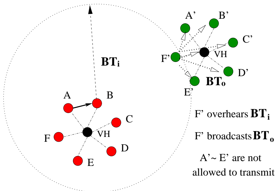
Figure 2.25: The BT_0 collision avoidance mechanism according to the game theoretic DSA-driven protocol [69].
