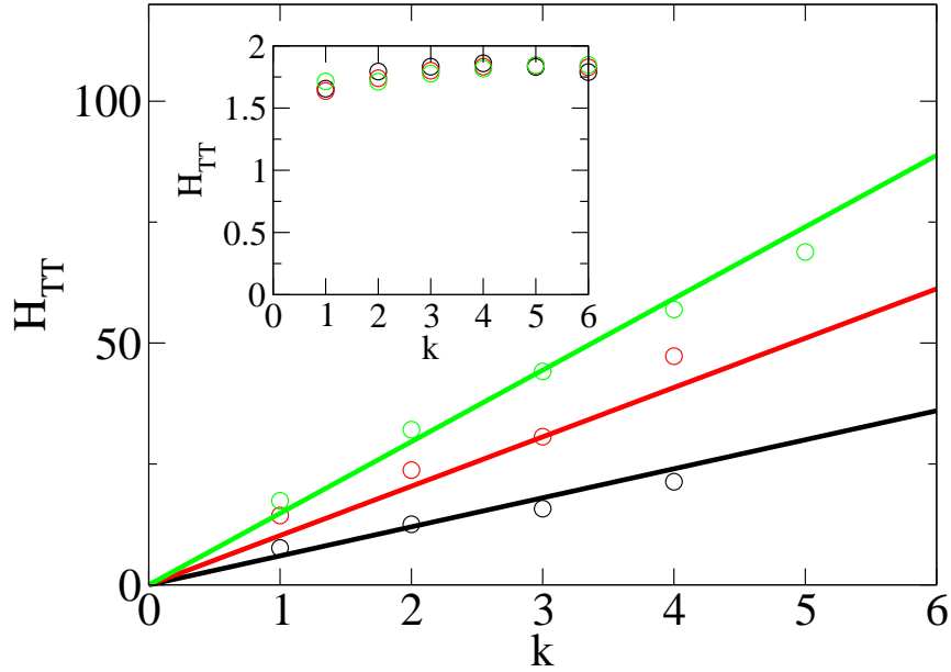
Figure 3.22: Numerical computation of H(\mathbf{r}_T|\mathbf{r}_T) for critical 3D percolation networks ( p = 0.2488 , compact case). The circle stand for numerical simulation, for a 10^3 network (black circles), 15^3 (red) and 20^3 (green). A fit in CkN^{d_w/d_f-1} (straight line) is performed, with the same fitting constant C for the three sizes. (Inset) supercritical 3D percolation networks ( p = 0.8 , non-compact case). Three network sizes are plotted, 10^3 (black), 15^3 (red) and 20^3 (green).
