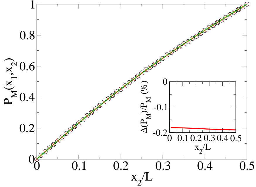
Figure 3.7: Encounter probability of two random walkers on the interval [0, 1] , starting in (x_1, x_2) , where x_1 = 0.5 , and x_2 \in [0, 0.5] . Black circles stand for simulations results, red crosses for the approximate expression of equation (3.23) and the green line for the exact result given by equation (3.22). (Inset) Relative difference between the approximate and the exact results in %. The relative error is of the same order of magnitude for all x_2 (below 0.2 %).
