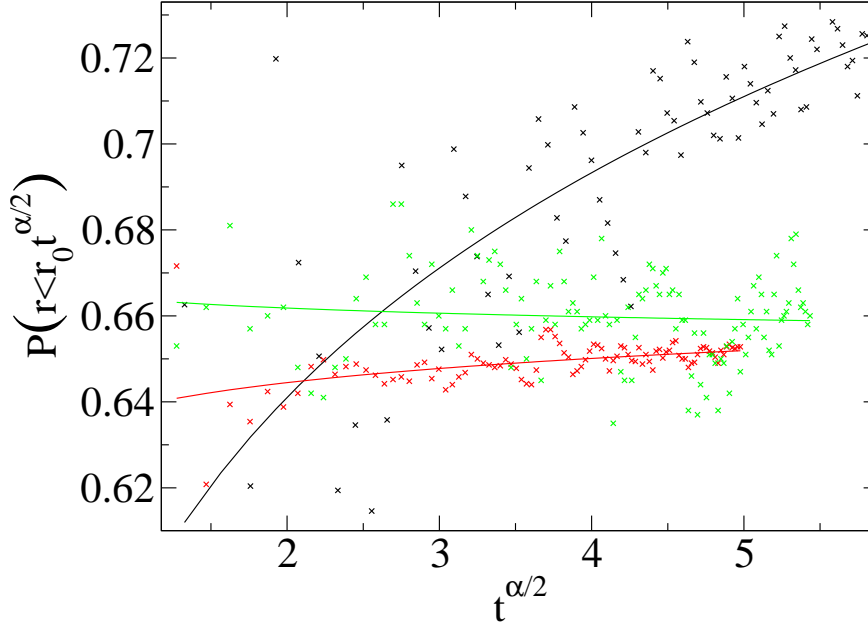
Figure 2.11: Probability to be in a growing shell of radius r_0 t^{\alpha/2} as function of t^{\alpha/2} for the three simulated sets (arbitrary units). This analysis is based on the previously fitted values of \alpha . The 2D critical percolation cluster (black \times ) produces d - f_f \simeq 0.11 , i. e. d_f \simeq 1.89 (exact value 91/48 \simeq 1.896 ). The CTRW set (red \times ) gives d - d_f \simeq 0.01 instead of 0, and the fBm set (green \times ) leads to d - d_f \simeq -0.004 instead of 0.
