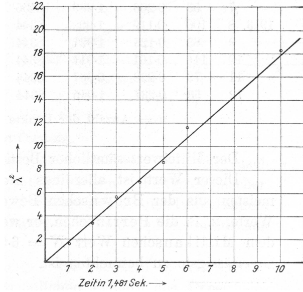
Figure 2.3: Mean square displacement obtained from a single trajectory by Nordlund [149].
