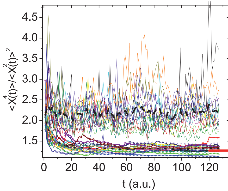
Figure 2.24: Displacement (upper curves) and maximal excursion (lower curves) ratio for lipid granules diffusing in S. pombe recorded by video tracking. Each curve correspond to a given lipid granule, and the overlaid black thick line stand for the average over the different lipid granules. The expected Brownian values are 2 for the displacement ratio, and 1.49 for the maximal excursion ratio. The experimental displacement ratio seems to be above the Brownian value, while the experimental maximal excursion ratio is under the expected value for a Brownian motion.
