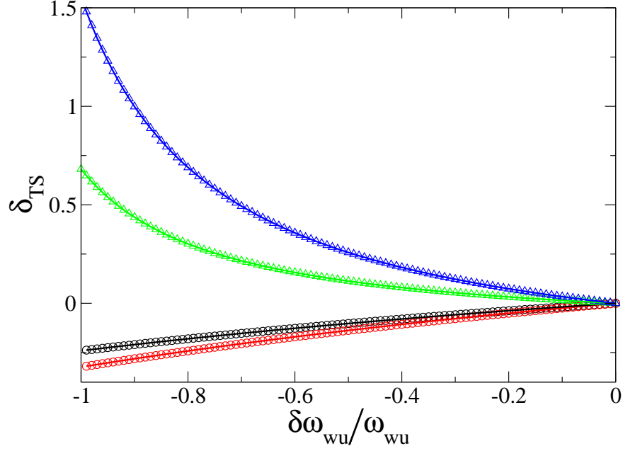
Figure 3.26: Relative variation of the MFPT \delta_{TS} as a function of the u \rightarrow w link perturbation, for given T , u and w sites. Two different starting sites S are chosen for each network (one color for each S ): circles stand for 2D critical percolation clusters (red and black) and triangles for (3,3)-flowers of generation 3 (green and blue).
