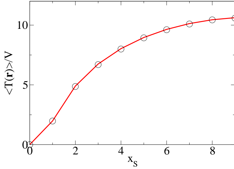
Figure 28: Mean first-passage time for a 10 \times 10 -large network with reflective boundaries, where \mathbf{r}_s = (x_S, 0) , \mathbf{r}_T = (0, 0) , \mathbf{e}_S = (1, 0) , with x_S \in [0, 9] . Here \epsilon = -0.04 and \delta = 0.32 . The black circles stand for numerical simulations, the red line for theoretical result of equation (164).
