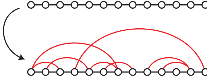
Figure 1.21: Creation of a Kozma network starting from a 1D Euclidian network.
