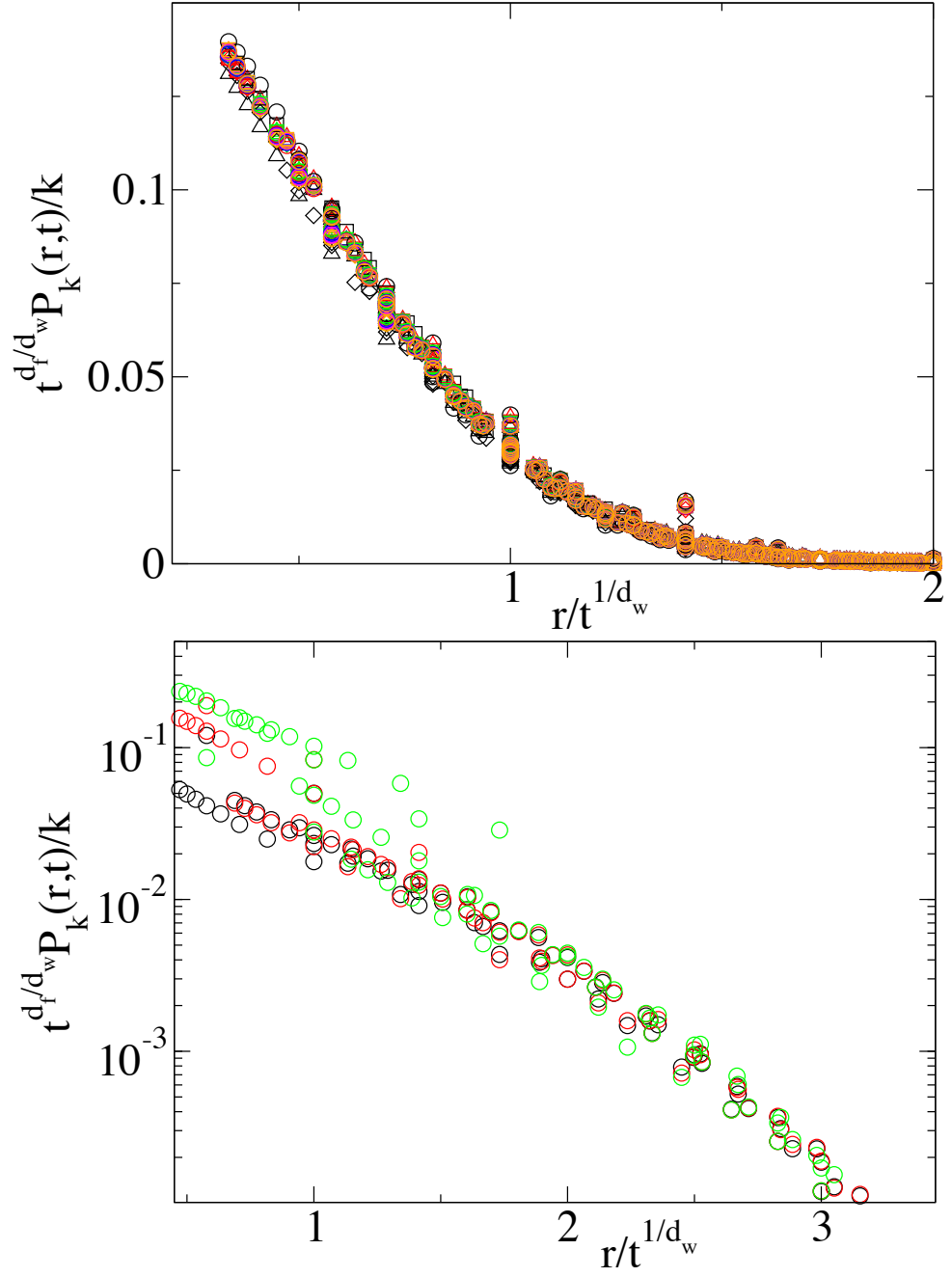
Figure 3.14: Plot of the propagator P(\mathbf{r}_T, n|\mathbf{r}_S) for non compact explorations. (Upper plot) Supercritical 3D percolation networks ( p = 0.8 ). Black, red, green, blue, magenta and orange symbols stand respectively for target connectivities k(\mathbf{r}_T) = 1, 2, 3, 4, 5 and 6 . Circles, triangles, diamonds and squares stand respectively for networks of size 20^3, 25^3, 30^3 and 40^3 . (Lower plot) (2, 2, 2) -flowers. Black, red and green circles stand respectively for target connectivities k(\mathbf{r}_T) = 2, 6 and 18 .
