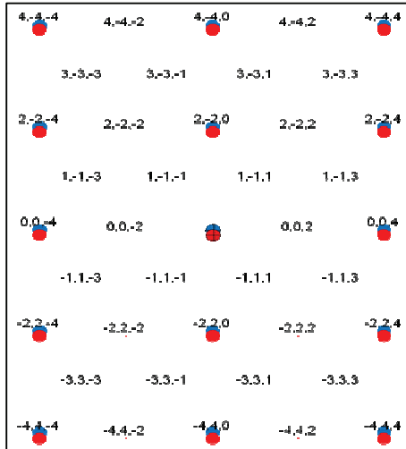
Figure IV-15: simulation of electron diffraction pattern of ferritic matrix (blue) in \langle 110 \rangle direction and Fe 2 SiTi extra spots (red)
