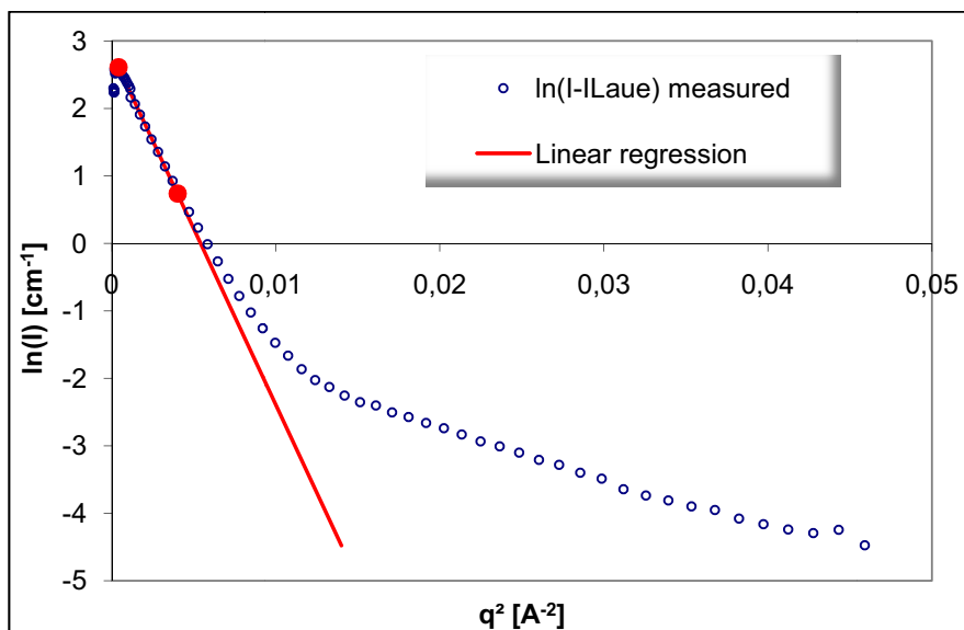
Figure II-26: Evolution of \ln(I) as a function of q^2 . The beginning of the curve is taken as linear, using its slope for determining R_g
