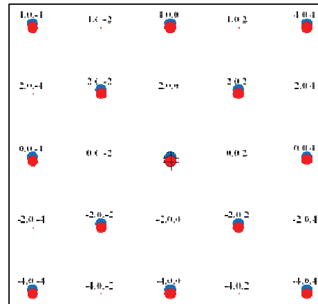
Figure IV-16: simulation of electron diffraction pattern of ferritic matrix (blue) in \langle 100 \rangle direction and Fe 2 SiTi extra spots (red)
