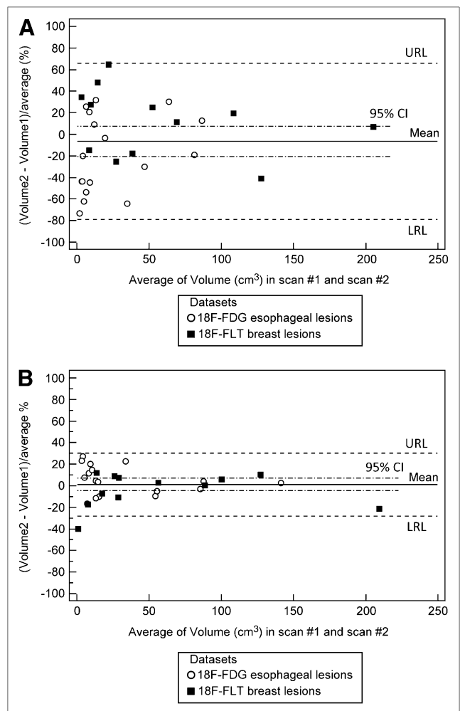
FIGURE 4. Bland-Altman plots of TV using adaptive thresholding (A) and TV using FLAB (B) for both ^{18}F -FDG and ^{18}F -FLT lesions. Lines show combined mean, 95% CI, and upper and lower reproducibility limits. Individual values for ^{18}F -FDG and ^{18}F -FLT lesions are shown in Tables 2 and 3, respectively. LRL = lower reproducibility limit; URL = upper reproducibility limit.
