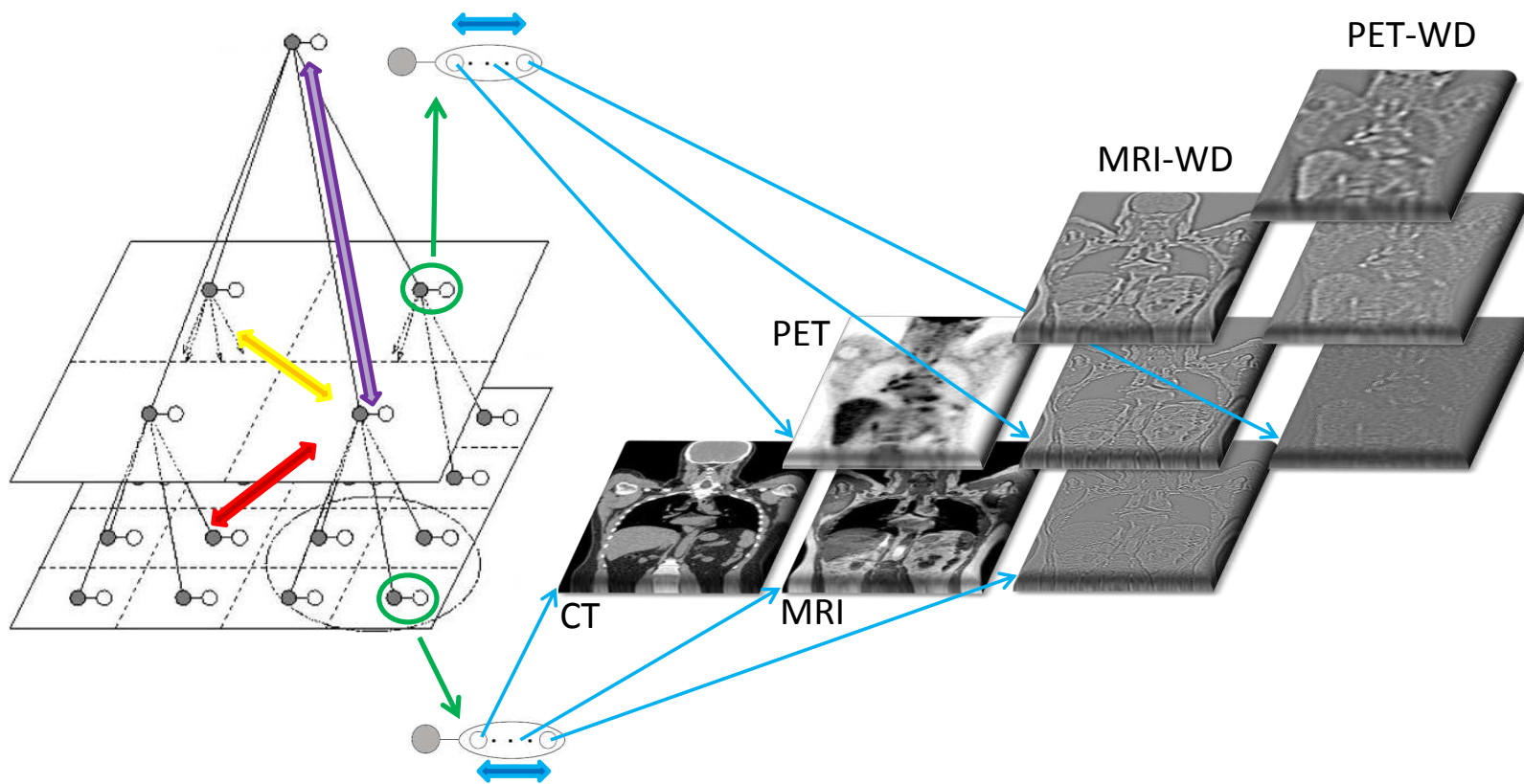
Fig.5: illustration of the multi observation, multi scale framework
