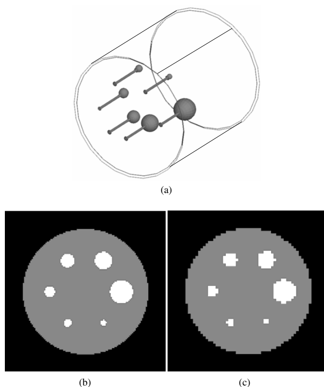
Figure 2. (a) A graphical representation of the IEC phantom, and the central slice of the digital IEC phantom used in the generation of the simulated datasets (b) with 2 \times 2 \times 2 \text{ mm}^3 and (c) 4 \times 4 \times 4 \text{ mm}^3 .
