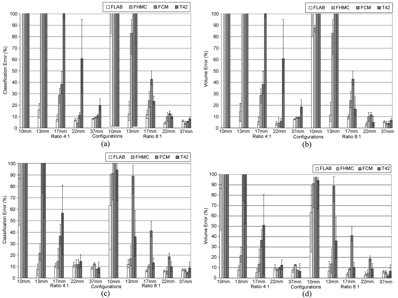
Fig. 6. Comparison of performances for FLAB, FHMC, FCM, and T42 on data reconstructed with (a) classification errors and (b) volume errors, for 64 mm 3 and (c) classification errors and (d) volume errors, for 8 mm 3 voxels. The top of the error bar is the result concerning the worst statistical quality images (1 min acquisition), the medium one concerns the medium quality (2 min acquisition), and the lowest one corresponds to the superior statistical quality (5 min acquisition).
