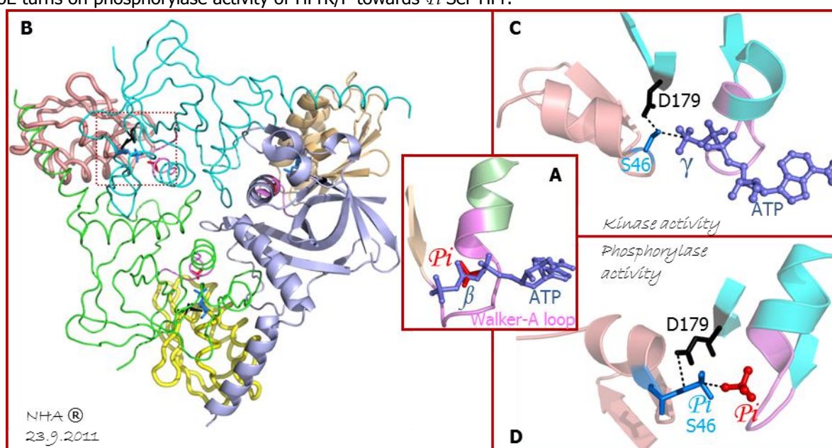
In fig. 13B , HPr was presented in yellow, wheat and salmon color, the rest are 3 chains of HPrK/P. The small dashed square was zoomed in fig. 12C (with HPr) and fig. 12D (with P_i -Ser-HPr)
