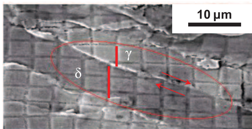
Figure II.4. A clear example of interphase boundary sliding in a 2205 duplex stainless steel deformed to 0.15 at 1050°C and 1s -1 [14].
