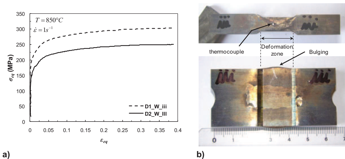
Figure IV.22. a) Comparison between the macroscopic stress strain curves of the D1_W and D2_W microstructures obtained under plane strain compression at 850°C and 1s -1 up to a reduction of 30%; b) pictures showing a top view and a front view of a deformed plane strain compression specimen.
